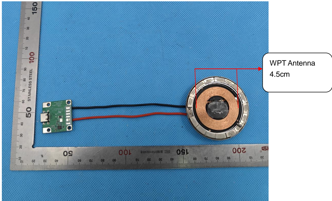
OPEN VIEW OF EUT (FIGURE 4)
