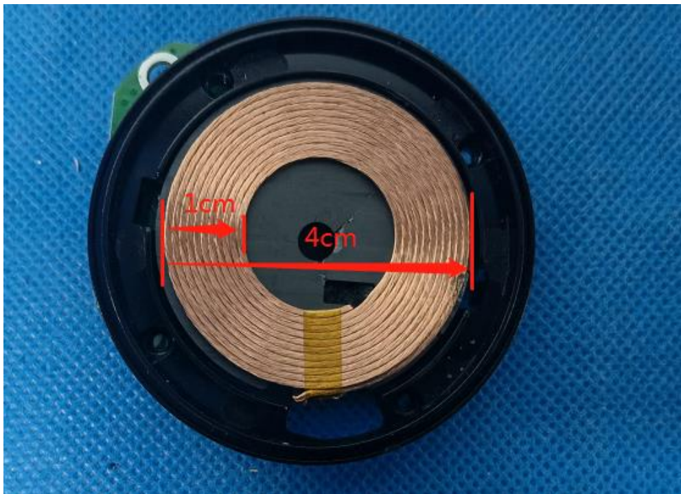
INTERNAL VIEW OF EUT (FIGURE 6)
