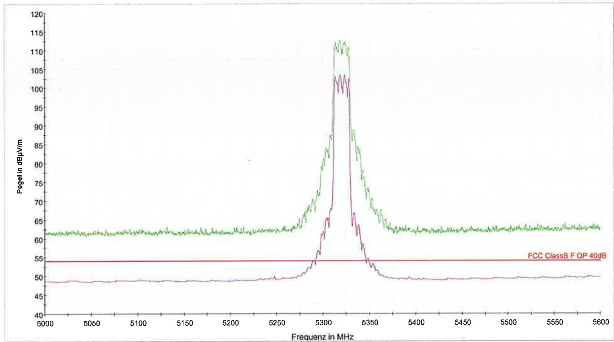
PK+_MAXH@S810_Bandedge [S810_5_20_CH64_Bandedge.Result:2] AVG_MAXH@S810_Bandedge [S810_5_20_CH64_Bandedge.Result:4] FCC ClassB F QP 40dB [..EMI radiated]
