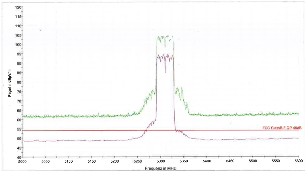
— PK+_MAXH@S810_Bandedge [S810_5_40_CH6064_Bandedge.Result:2] — AVG_MAXH@S810_Bandedge [S810_5_40_CH6064_Bandedge.Result:4] — FCC ClassB F QP 40dB [..EMI radiated]
