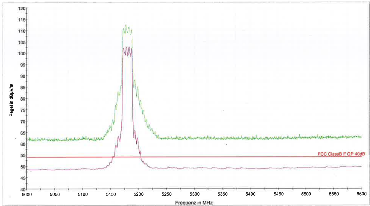
PK+_MAXH@S810_Bandedge [S810_5_20_CH36_Bandedge.Result:2] AVG_MAXH@S810_Bandedge [S810_5_20_CH36_Bandedge.Result:4] FCC ClassB F QP 40dB [..IEMI radiated]
