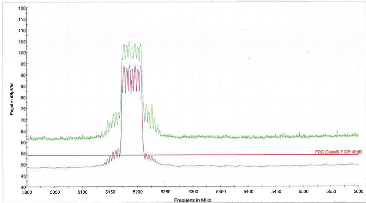
PK+_MAXH@S810_Bandedge [S810_5_40_CH3640_Bandedge.Result:2] — AVG_MAXH@S810_Bandedge [S810_5_40_CH3640_Bandedge.Result:4] FCC ClassB F QP 40dB [..EMI radiated]
