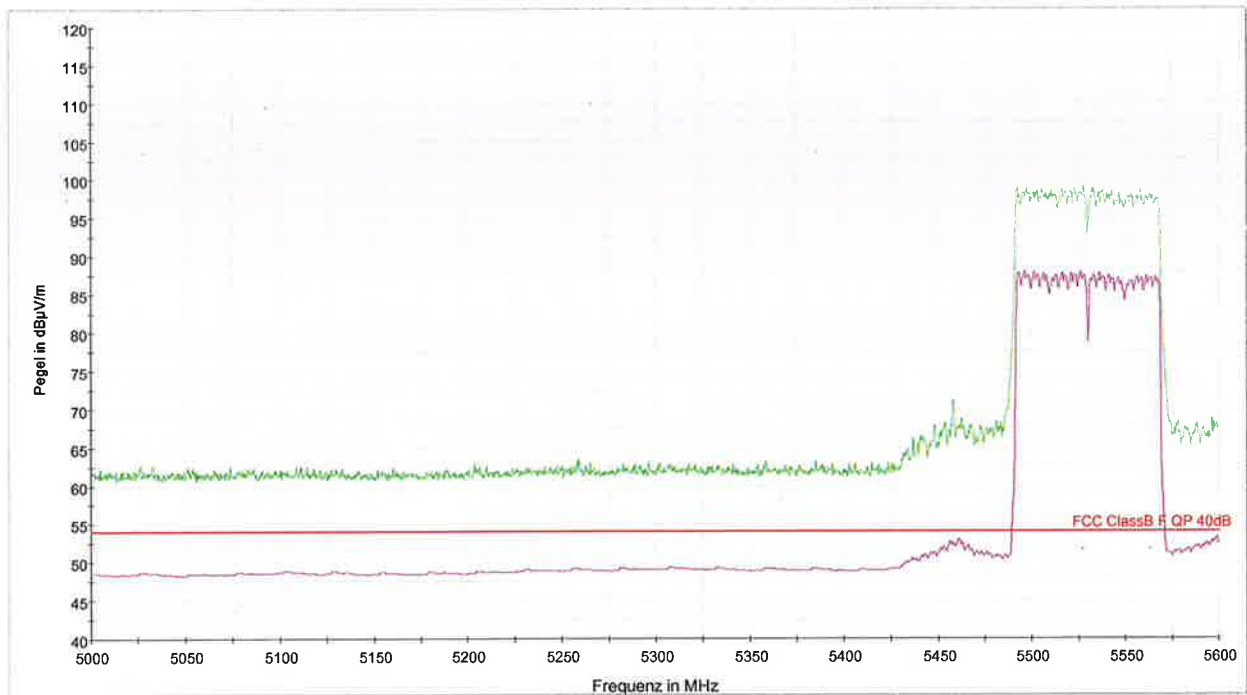
PK+_MAXH@S810_Bandedge [S810_5_80_CH100112_Bandedge.Result:2] AVG_MAXH@S810_Bandedge [S810_5_80_CH100112_Bandedge.Result:4] FCC ClassB F QP 40dB [..\EMI radiated]
