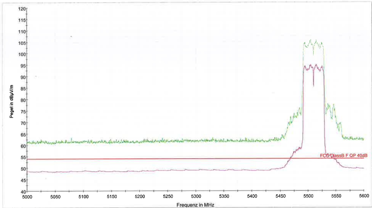
PK+_MAXH@S810_Bandedge [S810_5_40_CH100104_Bandedge.Result:2] — AVG_MAXH@S810_Bandedge [S810_5_40_CH100104_Bandedge.Result:4] FCC ClassB F QP 40dB [..EMI radiated]
