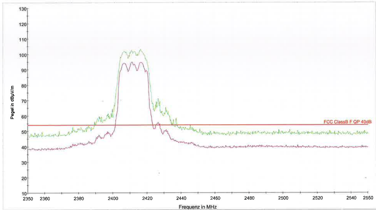
PK+ _MAXH@S810_2.4GHz_F1a [S810_2_4_20_CH1_F2.Result:2] AVG_MAXH@S810_2.4GHz_F1a [S810_2_4_20_CH1_F2.Result:4] FCC ClassB F QP 40dB [..\EMI radiated]
