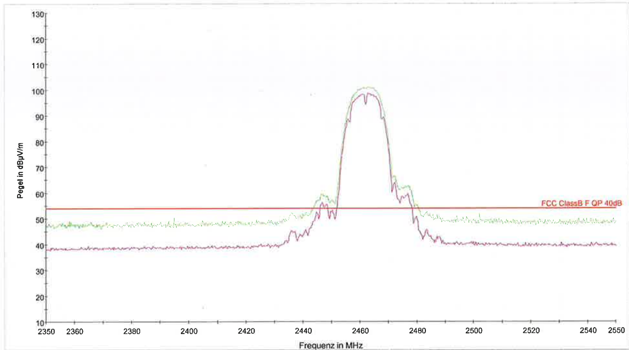
— PK+_MAXH@S810_2.4GHz_F1a [S810_2_4_DSSS_CH11_F2.Result:2] — AVG+_MAXH@S810_2.4GHz_F1a [S810_2_4_DSSS_CH11_F2.Result:4] — FCC ClassB F QP 40dB [„IEMI radiated“]
