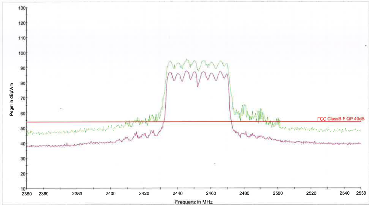
— PK+_MAXH@S810_2.4GHz_F1a [S810_2_4_40_CH7+11_F2.Result:2] — AVG_MAXH@S810_2.4GHz_F1a [S810_2_4_40_CH7+11_F2.Result:4] — FCC ClassB F QP 40dB [..EMI radiated]
