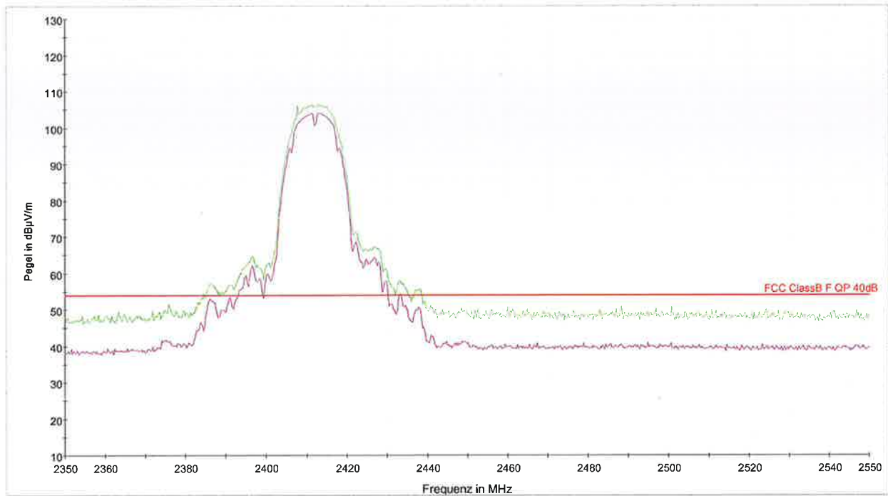
— PK+_MAXH@S810_2.4GHz_F1a [S810_2_4_DSSS_CH1_F2.Result:2] — AVG_MAXH@S810_2.4GHz_F1a [S810_2_4_DSSS_CH1_F2.Result:4] — FCC ClassB F QP 40dB [..EMI radiated]
