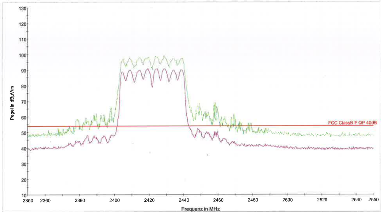
— PK+_MAXH@S810_2.4GHz_F1a [S810_2_4_40_CH1+5_F2.Result:2] — AVG_MAXH@S810_2.4GHz_F1a [S810_2_4_40_CH1+5_F2.Result:4] — FCC ClassB F QP 40dB [..IEMI radiated]
