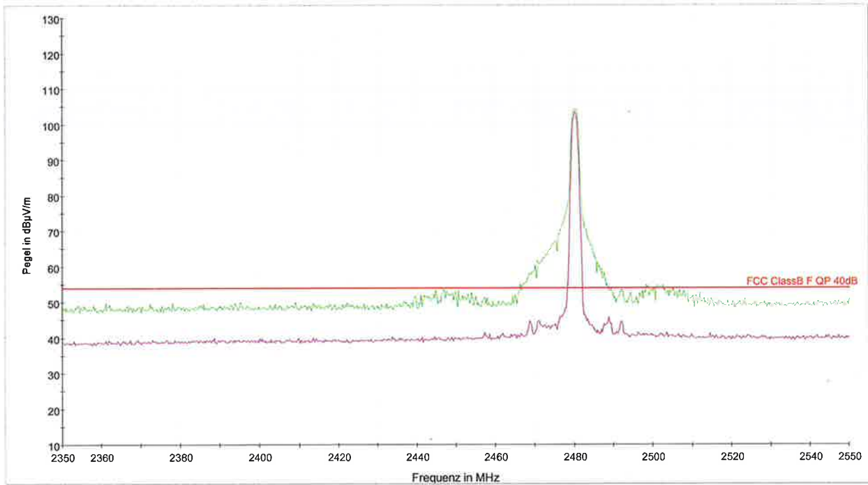
— PK+_MAXH@S810_2.4GHz_F1a [S810_BLE_CH39_F2.Result:2] — AVG_MAXH@S810_2.4GHz_F1a [S810_BLE_CH39_F2.Result:4] — FCC ClassB F QP 40dB [..EMF radiated]
