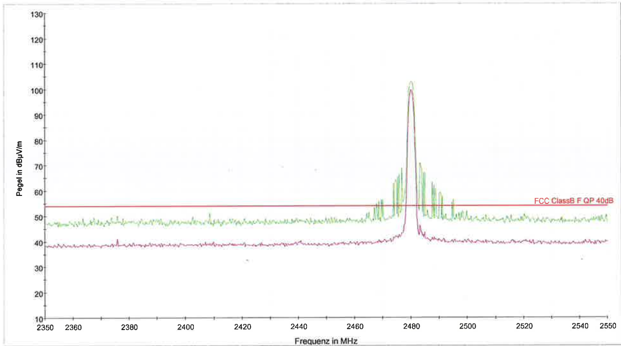
PK+_MAXH@S810_2.4GHz_F1a [S810_BT_EDR_CH78_F2.Result:2] AVG_MAXH@S810_2.4GHz_F1a [S810_BT_EDR_CH78_F2.Result:4] FCC ClassB F QP 40dB [..EMI radiated]
