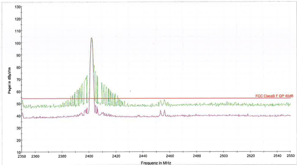
— PK+_MAXH@S810_2.4GHz_F1a [S810_BT_BDR_CH0_F2.Result:2] — AVG_MAXH@S810_2.4GHz_F1a [S810_BT_BDR_CH0_F2.Result:4] — FCC ClassB F QP 40dB [..IEMI radiated]
