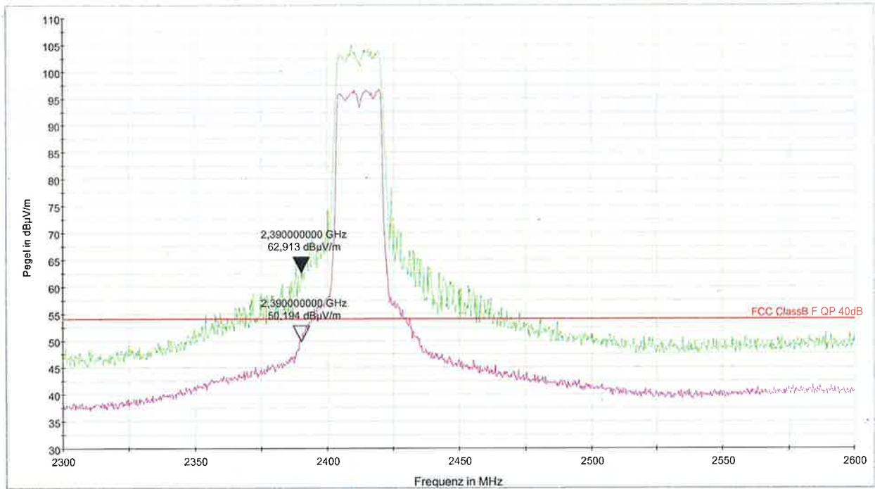
PK+_MAXH@S770_2.4GHz_F1a [S770_2_4_20_CH1_F2.Result:2] AVG_MAXH@S770_2.4GHz_F1a [S770_2_4_20_CH1_F2.Result:4] FCC ClassB F QP 40dB [..EMI radiated]
