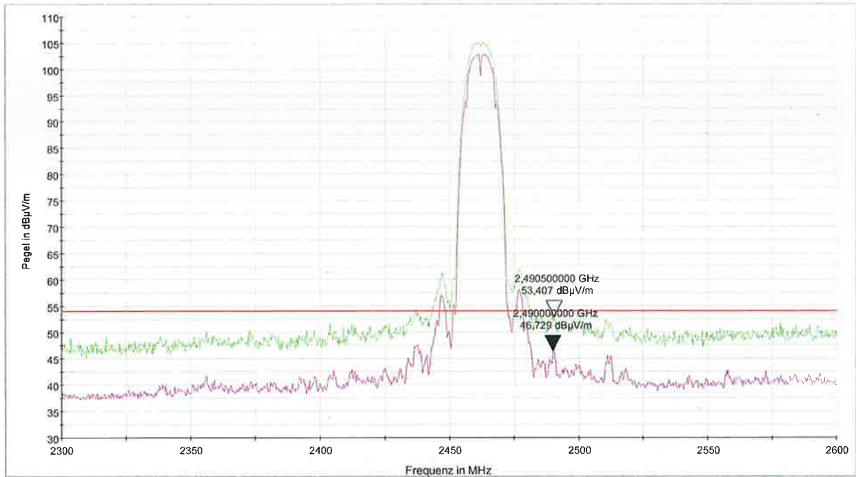
PK+_MAXH@S770_2.4GHz_F1a [S770_2_4_DSSS_CH11_F2.Result:2] AVG_MAXH@S770_2.4GHz_F1a [S770_2_4_DSSS_CH11_F2.Result:4] FCC ClassB F QP 40dB [..\EMI radiated]
