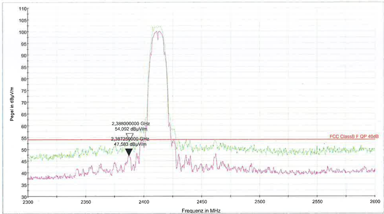
PK+_MAXH@S770_2.4GHz_F1a [S770_2_4_DSSS_CH1_F2.Result:2] AVG_MAXH@S770_2.4GHz_F1a [S770_2_4_DSSS_CH1_F2.Result:4] FCC ClassB F QP 40dB [.\EMI radiated]
