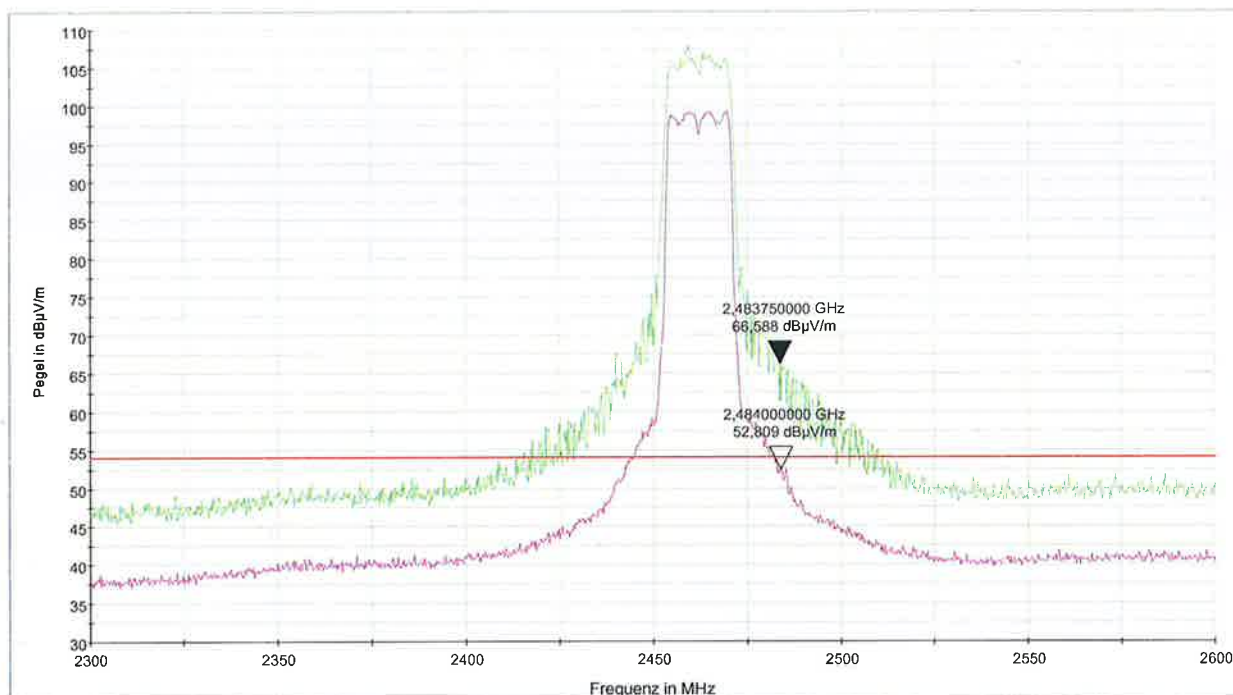
PK+ _MAXH@S770_2.4GHz_F1a [S770_2_4_20_CH11_F2a.Result:2] AVG_MAXH@S770_2.4GHz_F1a [S770_2_4_20_CH11_F2a.Result:4] FCC ClassB F QP 40dB [L\EMl radiated]
