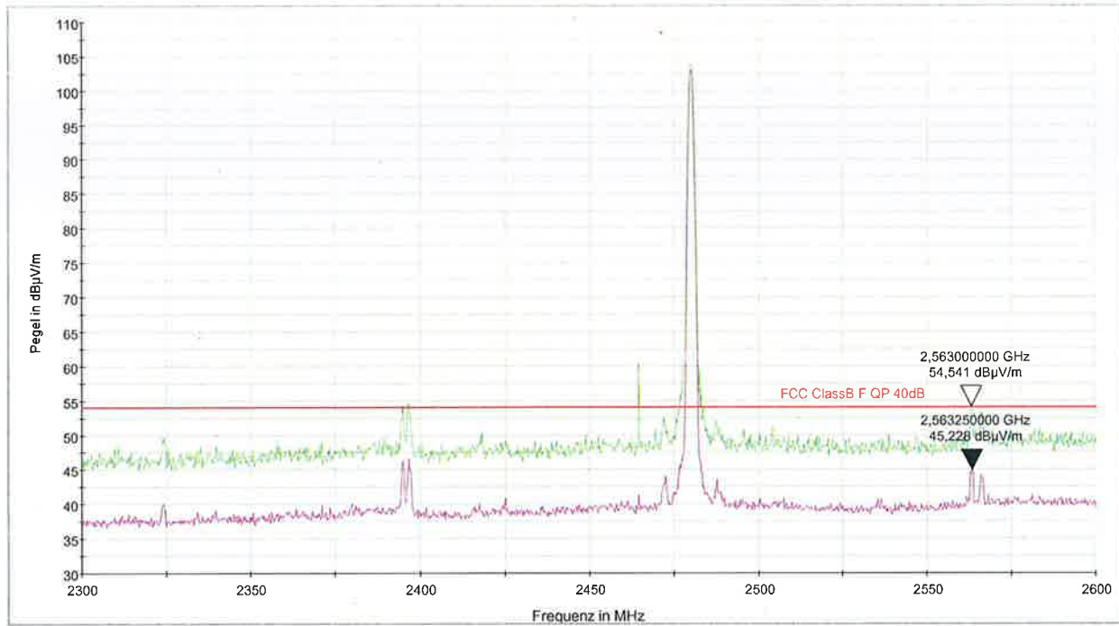
PK+_MAXH@S770_2.4GHz_F1a [S770_BLE_CH39_F2.Result:2] AVG_MAXH@S770_2.4GHz_F1a [S770_BLE_CH39_F2.Result:4] FCC ClassB F QP 40dB [„\EMI radiated“]
