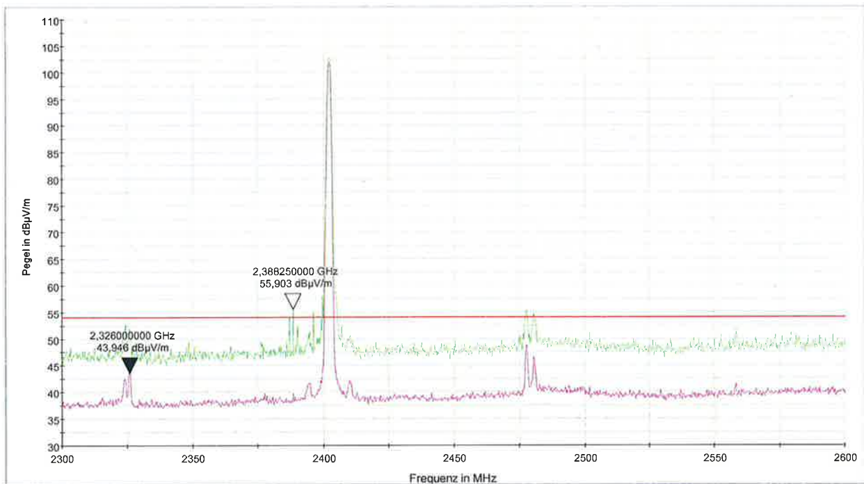
PK+_MAXH@S770_2.4GHz_F1a [S770_BT_BDR_CH0_F2.Result:2] AVG_MAXH@S770_2.4GHz_F1a [S770_BT_BDR_CH0_F2.Result:4] FCC ClassB F QP 40dB [..EMI radiated]
