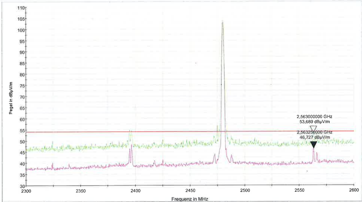
PK+_MAXH@S770_2.4GHz_F1a [S770_BT_BDR_CH78_F2.Result:2] AVG_MAXH@S770_2.4GHz_F1a [S770_BT_BDR_CH78_F2.Result:4] — FCC ClassB F QP 40dB [L\EMI radiated\]
