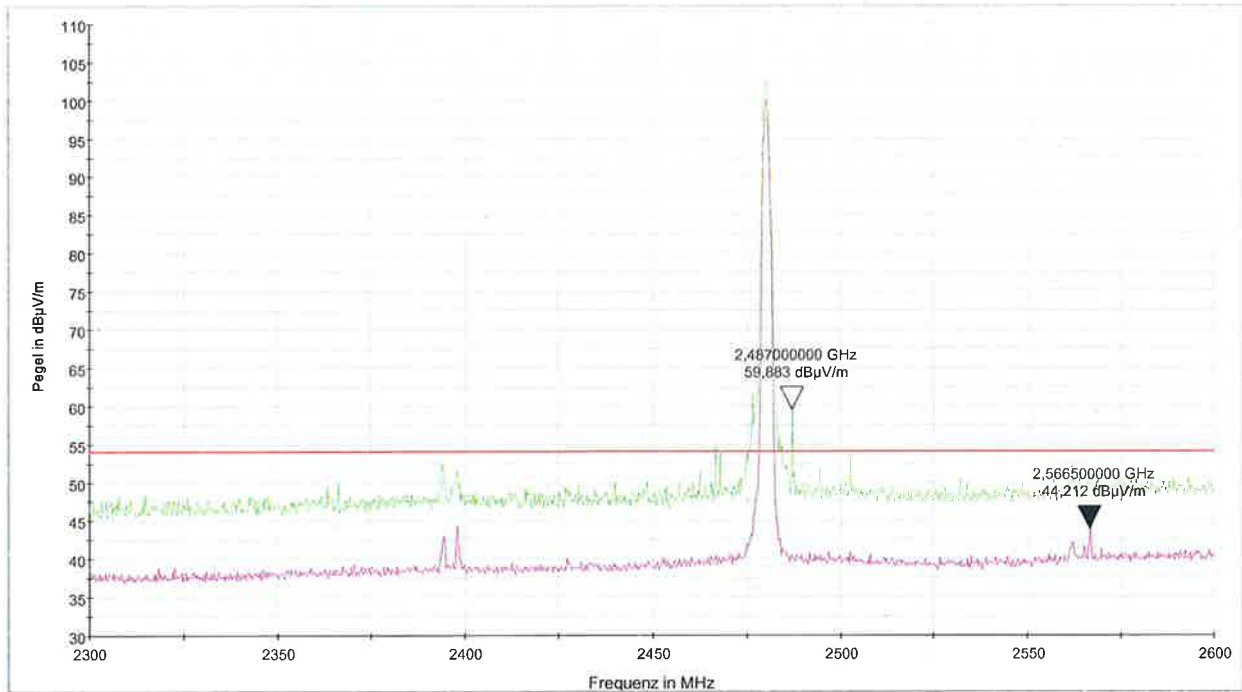
PK+_MAXH@S770_2.4GHz_F1a [S770_BT_EDR_CH78_F2.Result:2] AVG_MAXH@S770_2.4GHz_F1a [S770_BT_EDR_CH78_F2.Result:4] FCC ClassB F QP 40dB [..EMI radiated]
