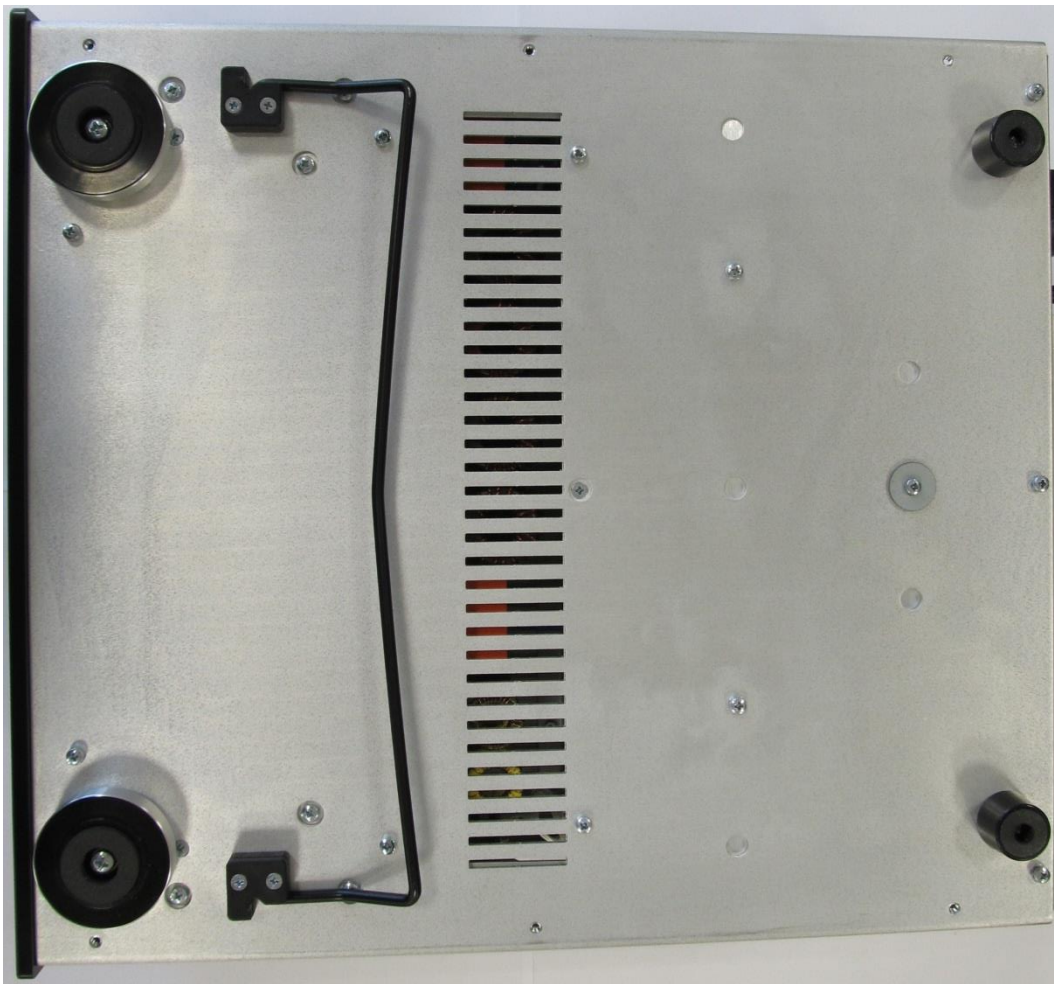
Fig.5 Bottom View
