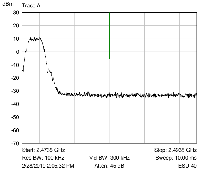
Graph 8: Upper Band Edge Plot
