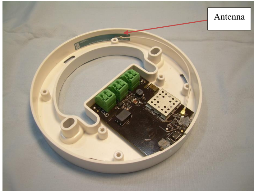
Photograph 13 – View of the EUT with the Housing Open
