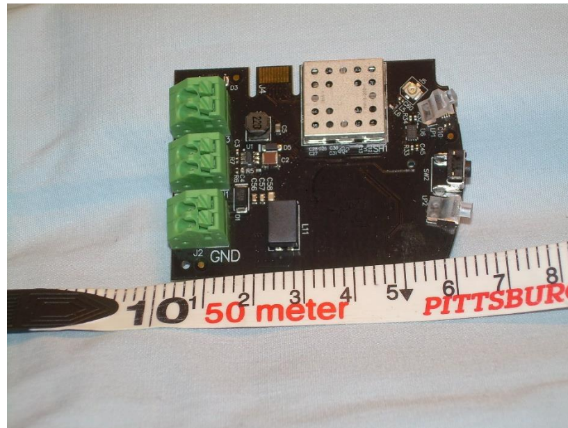
Photograph 14 – View of the Top Side of the PCB
