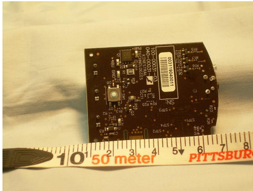
Photograph 15 – View of the Bottom Side of the PCB
