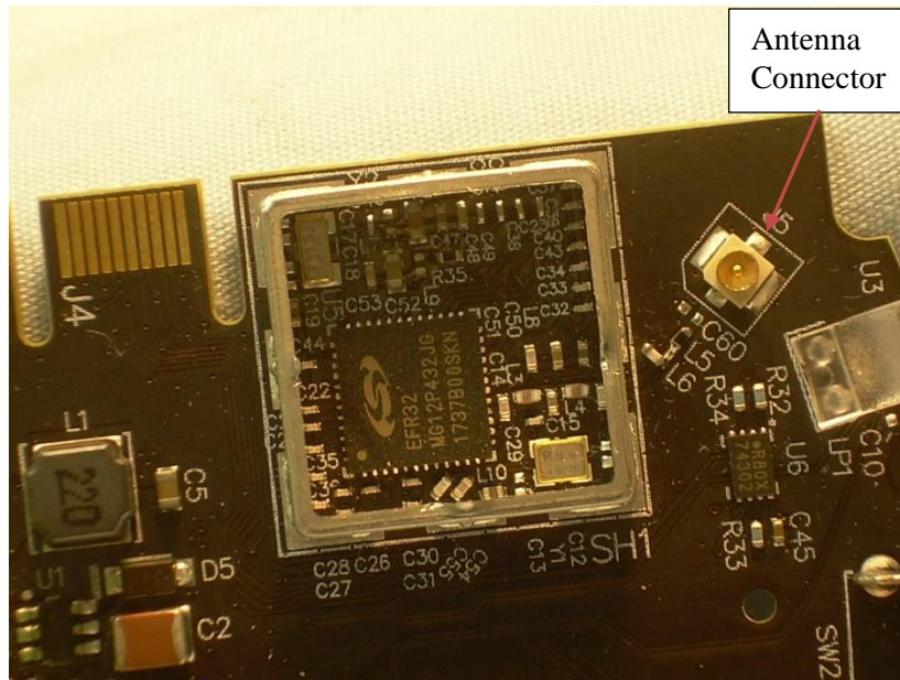
Photograph 16 – View of the Circuitry Under the RF Shield
