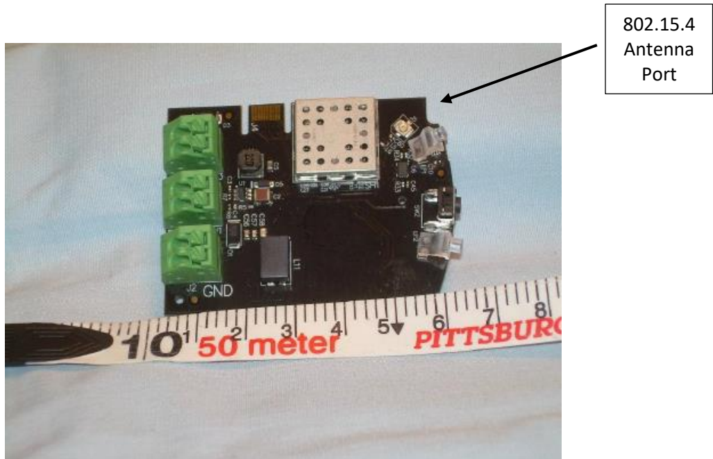
Photograph 1 – Top View of the PCB
