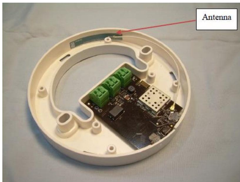
Photograph 4 – View of Antenna Placement
