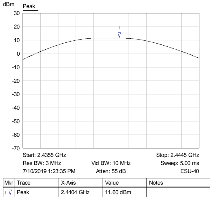
Graph 5: Middle Channel Output Power
