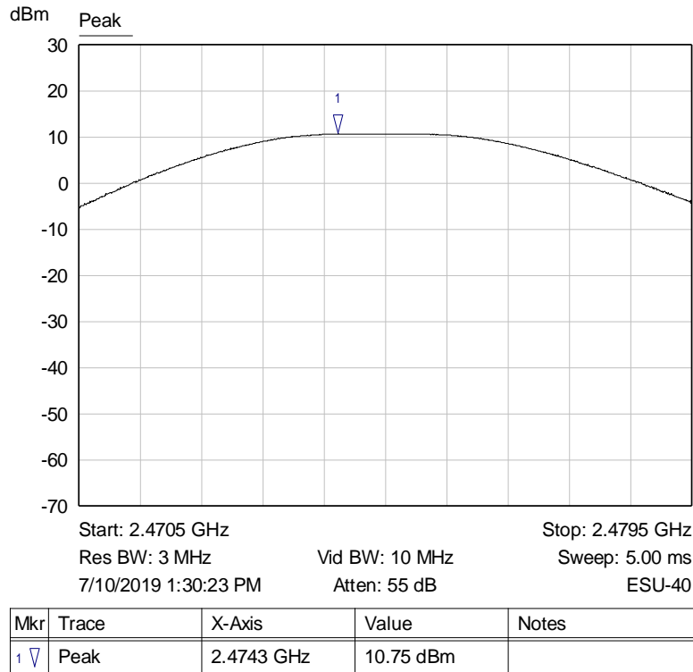
Graph 6: Highest Channel Output Power Plot
