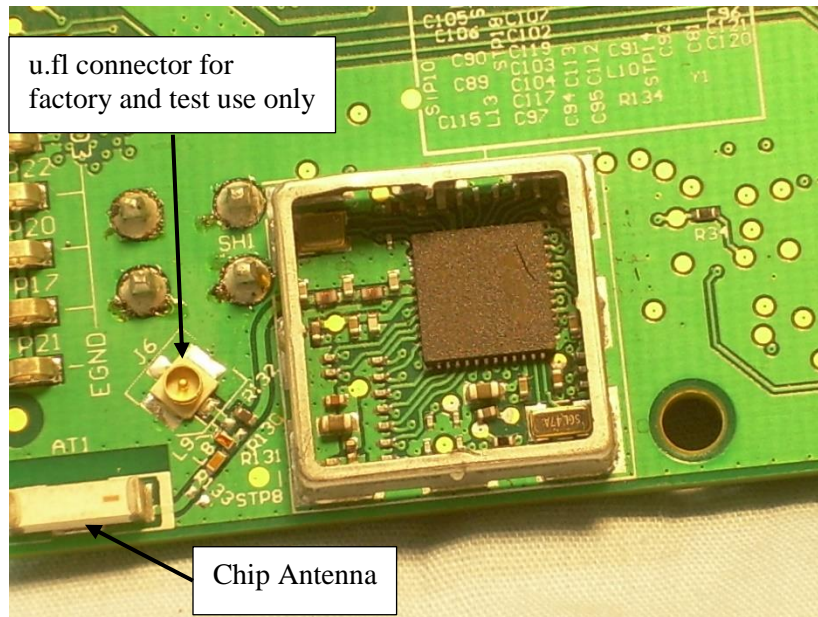
Photograph 15 – View of the Circuitry Under the RF Shield and Antenna
