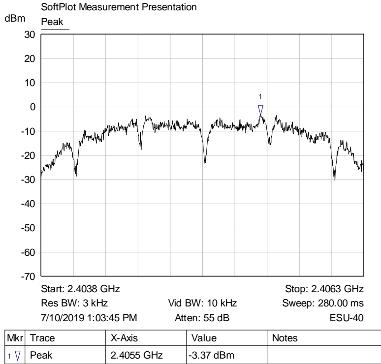
Graph 11: Lowest Channel 3 kHz PSD Plot
