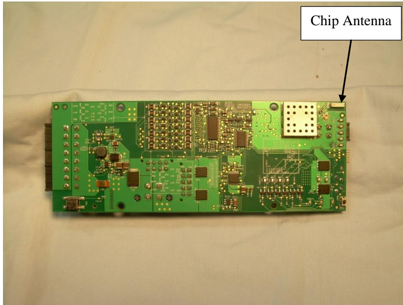
Photograph 14 – Back View of the PCB with RF Shield in Place
