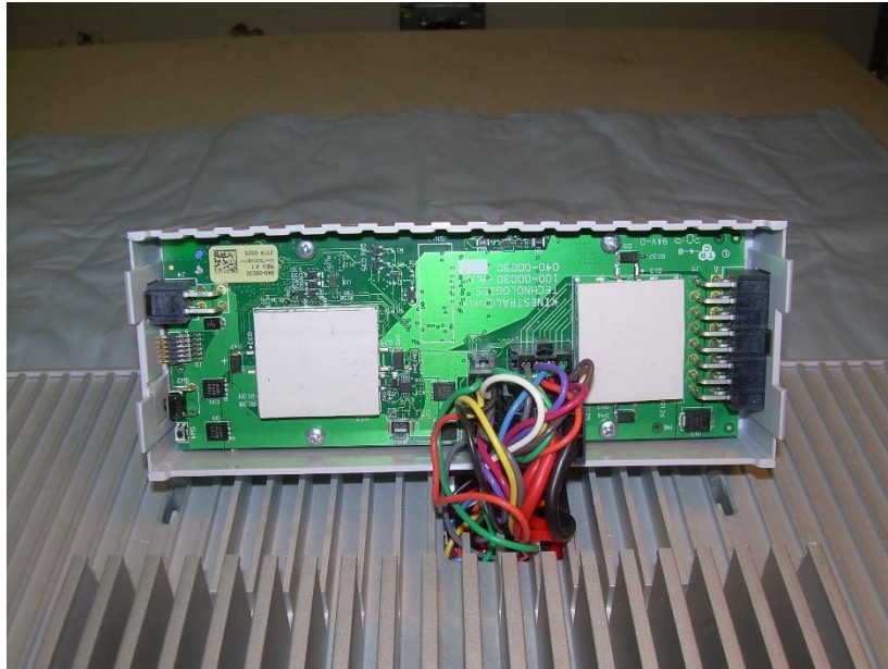
Photograph 11 – Internal View of the EUT PCB
