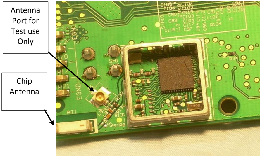
Photograph 3 – View of RF Circuitry
