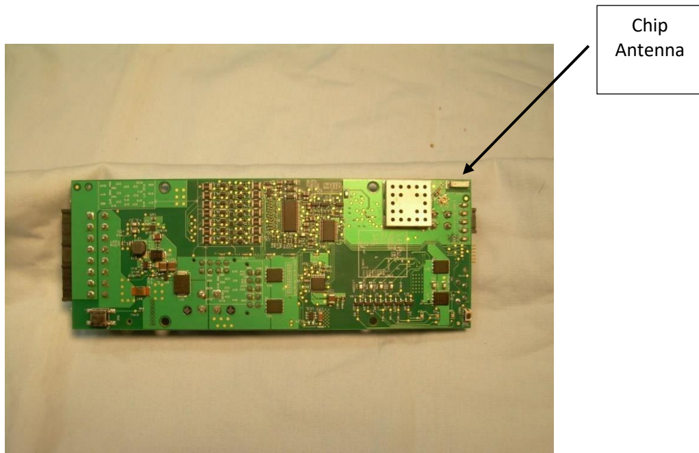
Photograph 1 – Bottom View of the PCB
