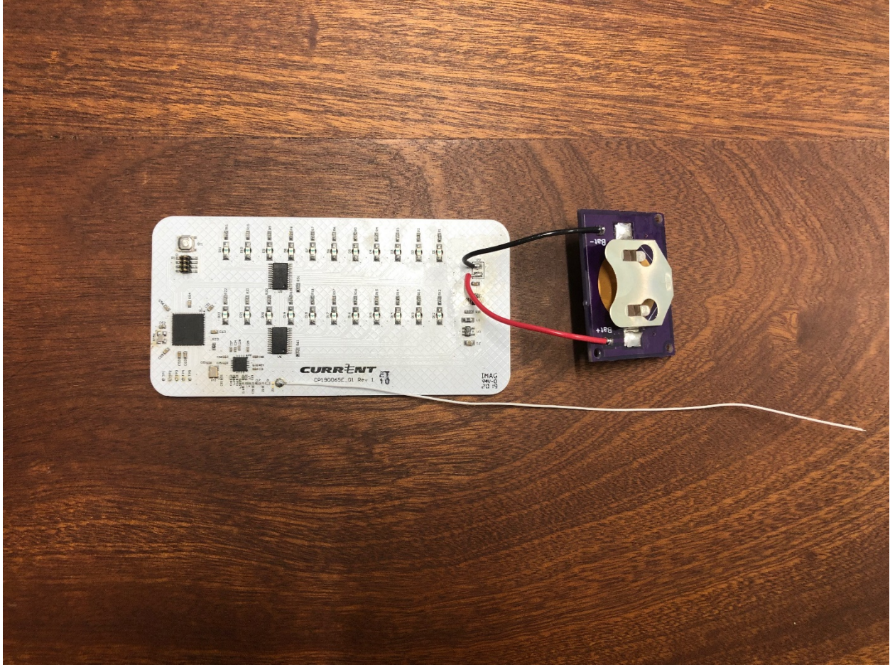
Figure 1: PCB View 1
