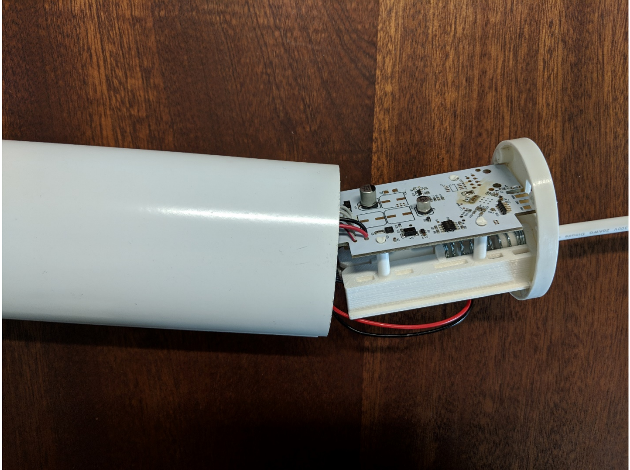
Figure 3: PCB Installed
