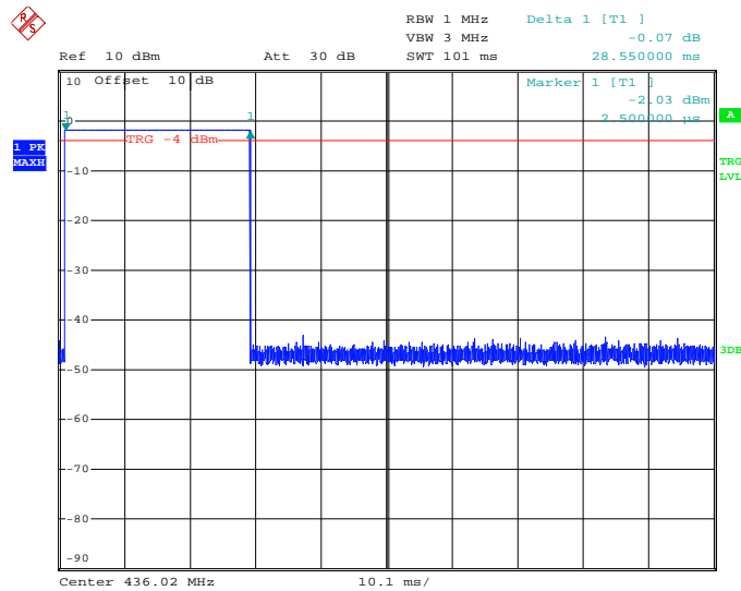
Figure 7.4.2-2: Periodic Operation – 5 Seconds – Low Channel
