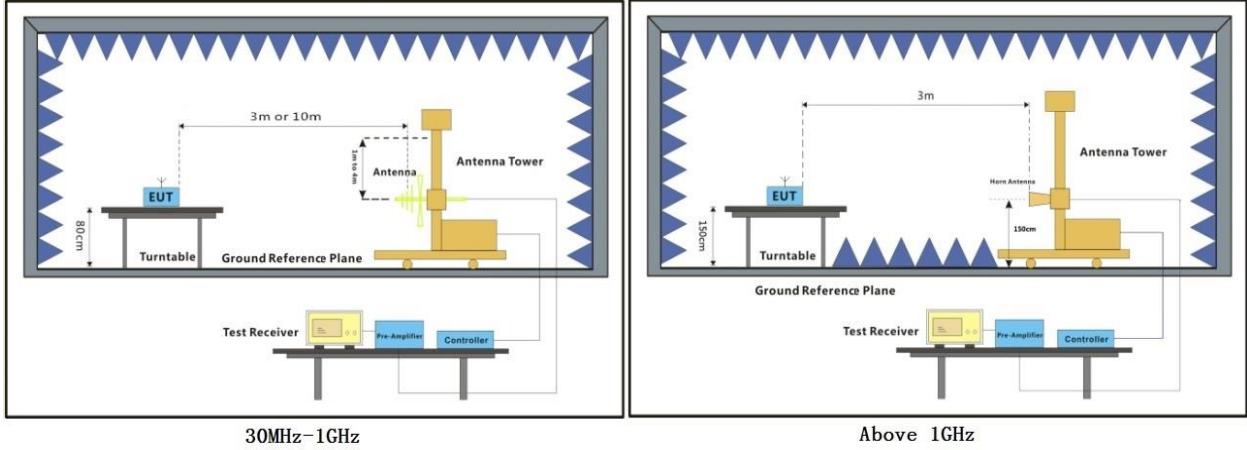
30MHz-1GHz
