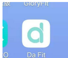
Test software
