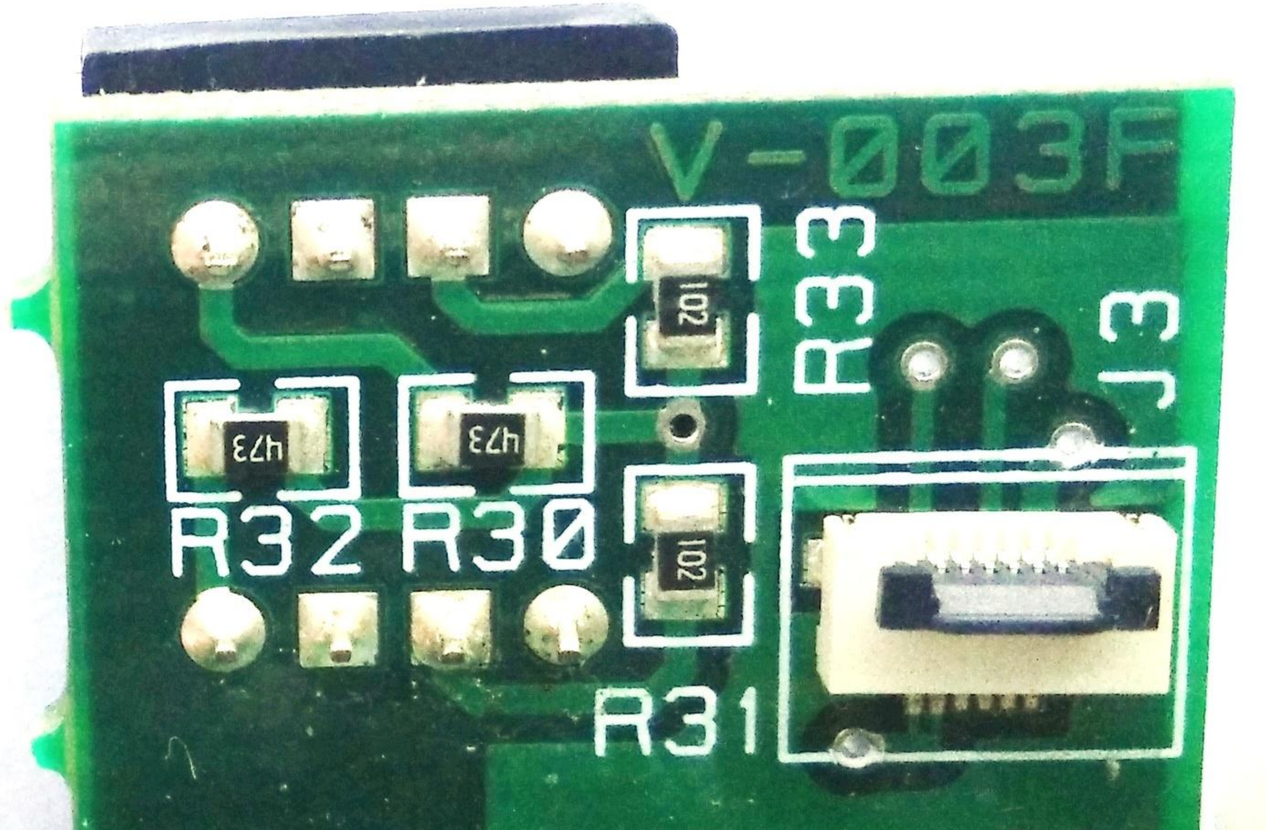
Vertical PCB (View 2)
