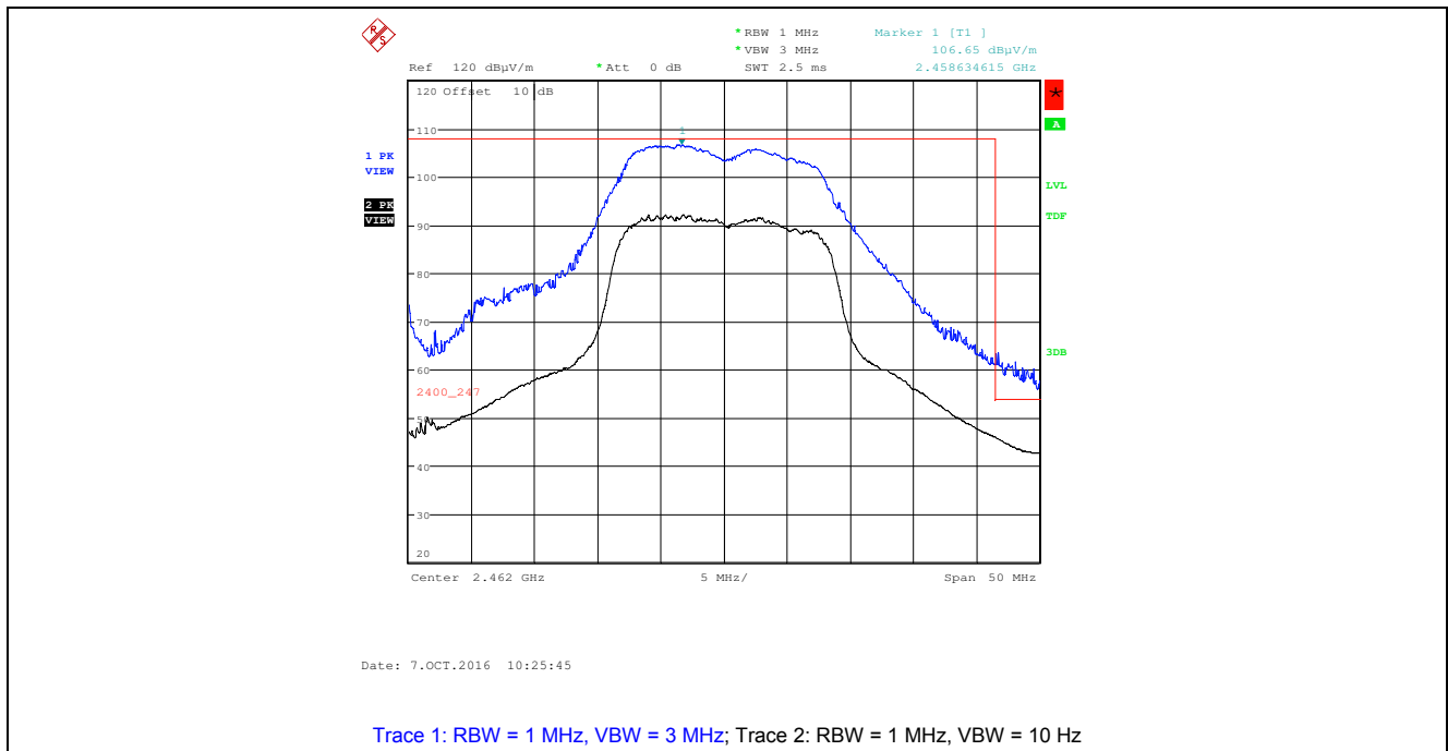
Plot 5.4.4.2.4. Band-Edge RF Radiated Emissions at 3 m, Vertical Polarization 802.11g, BPSK 6 Mbps, 2462 MHz, Power Setting 0
