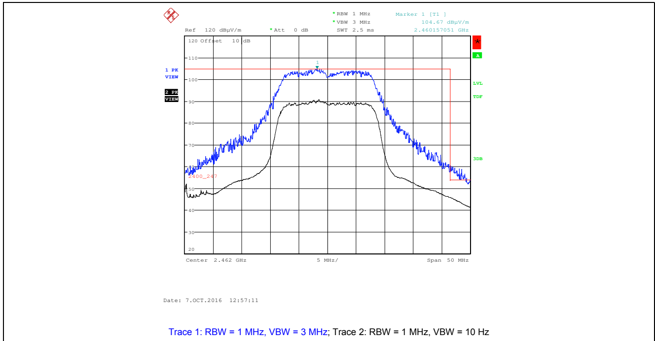
Plot 5.4.4.2.3. Band-Edge RF Radiated Emissions at 3 m, Horizontal Polarization 802.11g, BPSK 6 Mbps, 2462 MHz, Power Setting 0
