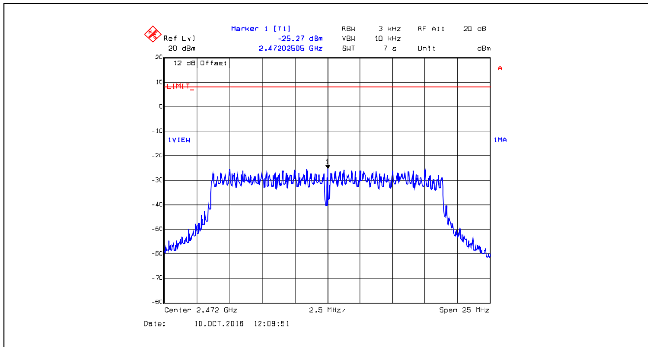
Plot 5.5.4.33. Power Spectral Density, 802.11n, 64-QAM 2/3 MCS 5, 52 Mbps, 2472 MHz, Power Setting 10
