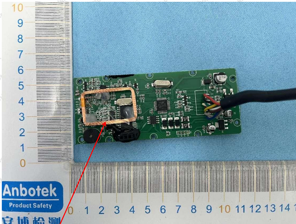
125kHz ANT
