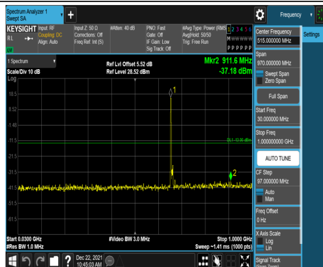
Band71-10MHz-QPSK-133172-1RB#0-Range3:30~1000MHz
