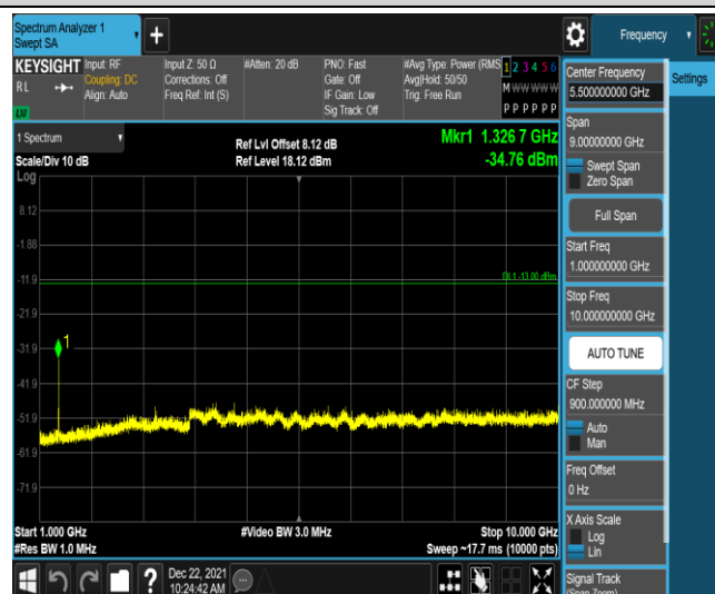
Band71-5MHz-16QAM-133147-1RB#0-Range4:1000~10000MHz
