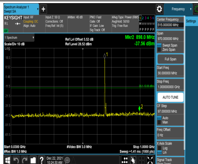
Band71-5MHz-16QAM-133147-1RB#0-Range3:30~1000MHz
