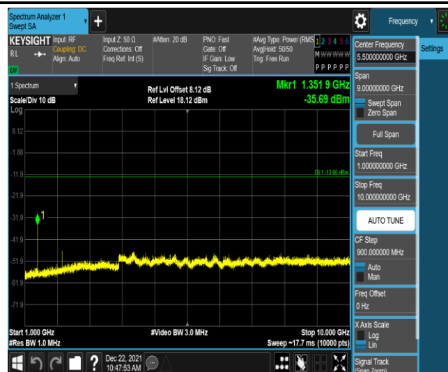
Band71-10MHz-16QAM-133297-1RB#0-Range4:1000~10000MHz
