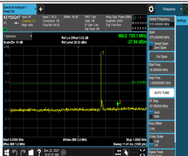
Band71-10MHz-16QAM-133297-1RB#0-Range3:30~1000MHz
