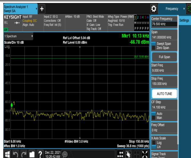
Band71-5MHz-QPSK-133447-1RB#0-Range1:0.009~0.15MHz
