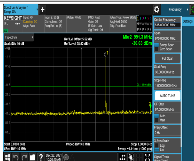
Band71-5MHz-16QAM-133297-1RB#0-Range3:30~1000MHz
