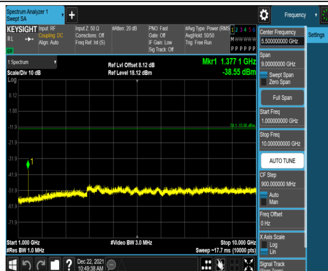
Band71-10MHz-16QAM-133422-1RB#0-Range4:1000~10000MHz
