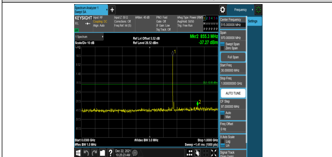
Band71-5MHz-QPSK-133297-1RB#0-Range3:30~1000MHz
