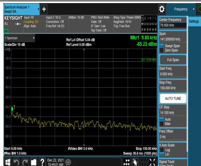
Band71-10MHz-16QAM-133422-1RB#0-Range1:0.009~0.15MHz
