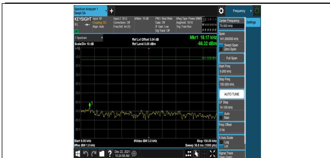
Band71-5MHz-QPSK-133297-1RB#0-Range1:0.009~0.15MHz
