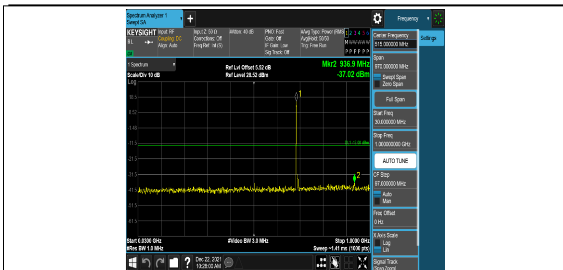
Band71-5MHz-16QAM-133447-1RB#0-Range3:30~1000MHz
