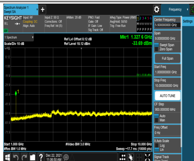
Band71-15MHz-QPSK-133197-1RB#0-Range4:1000~10000MHz
