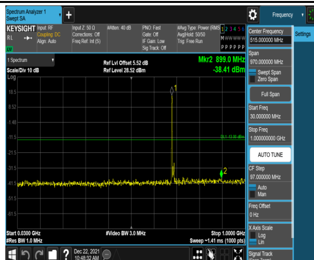
Band71-10MHz-QPSK-133422-1RB#0-Range3:30~1000MHz
