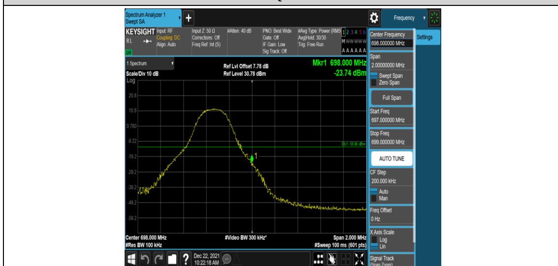
Band71-5MHz-16QAM-133447-1RB#24
