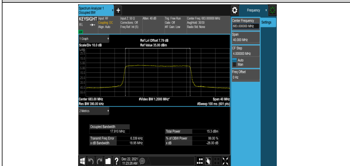
Band71-20MHz-QPSK-133322-100RB#0
