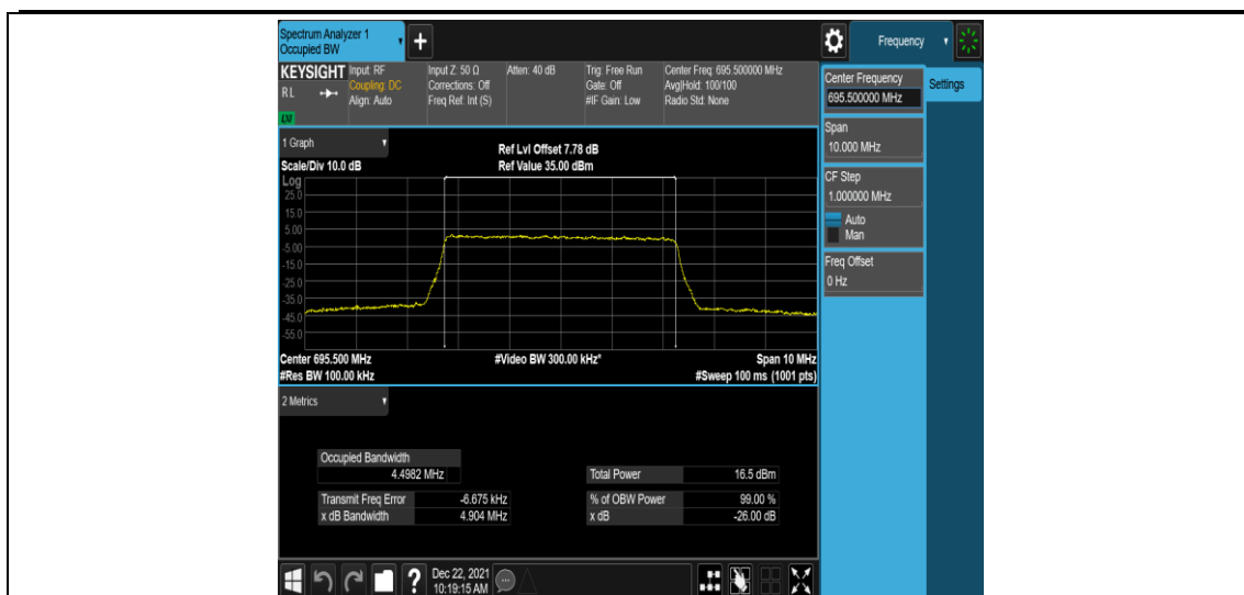
Band71-5MHz-16QAM-133447-25RB#0
