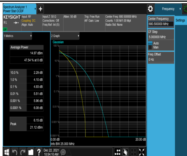
Band71-10MHz-QPSK-133297-50RB#0
