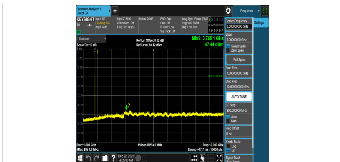
Band66-1.4MHz-16QAM-132322-1RB#0-Range4:1000~10000MHz
