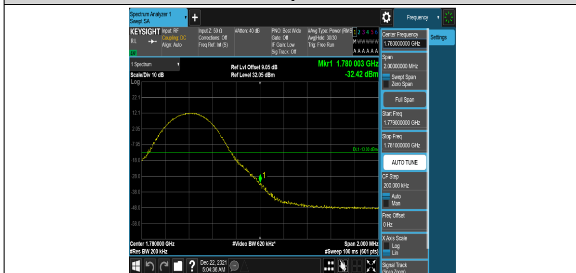
Band66-10MHz-16QAM-132622-1RB#49
