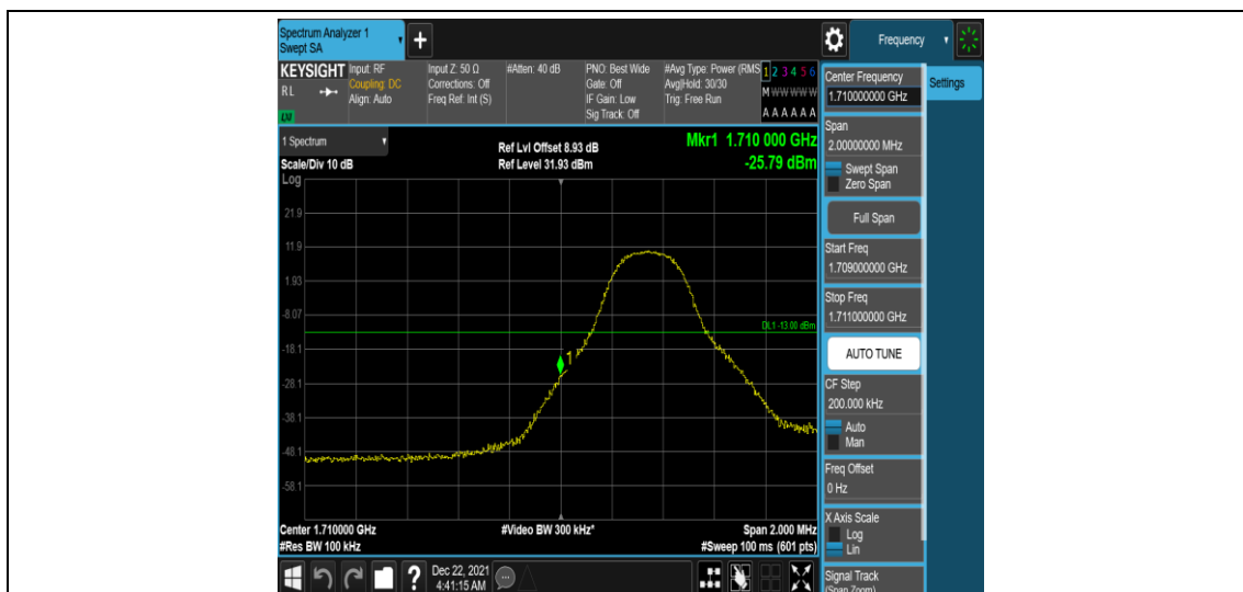
Band66-5MHz-QPSK-131997-1RB#0
