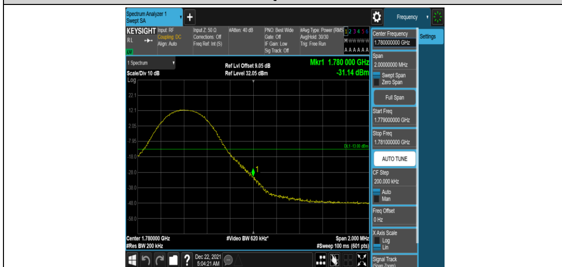
Band66-10MHz-QPSK-132622-1RB#49
