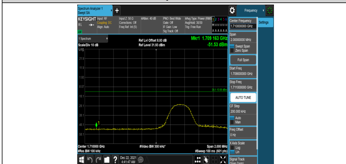
Band66-5MHz-QPSK-131997-1RB#24
