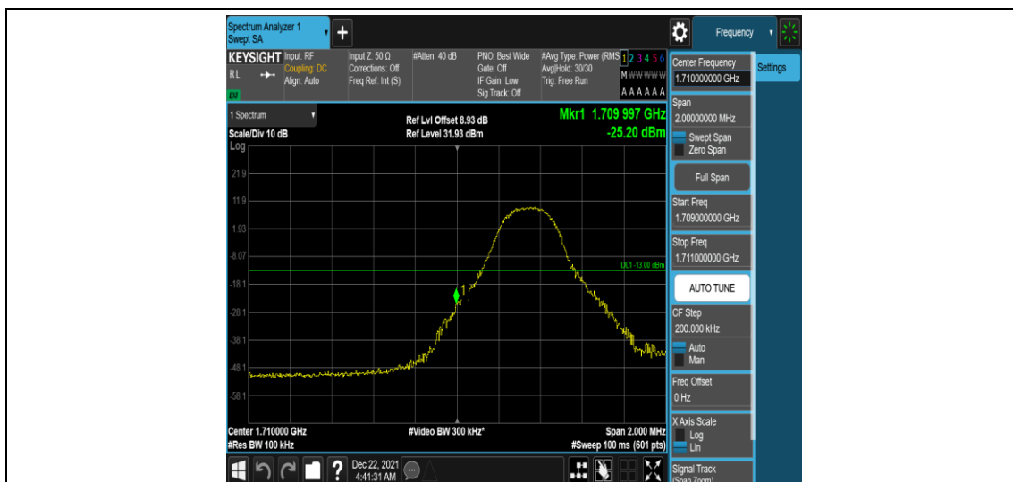
Band66-5MHz-16QAM-131997-1RB#0
