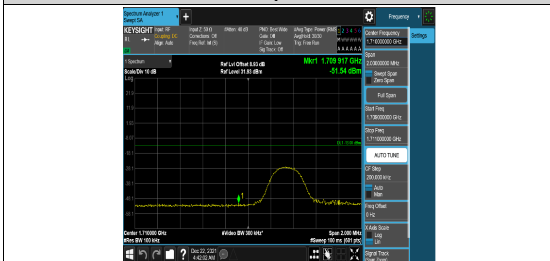
Band66-5MHz-16QAM-131997-1RB#24
