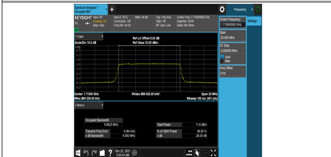
Band66-10MHz-16QAM-132022-50RB#0
