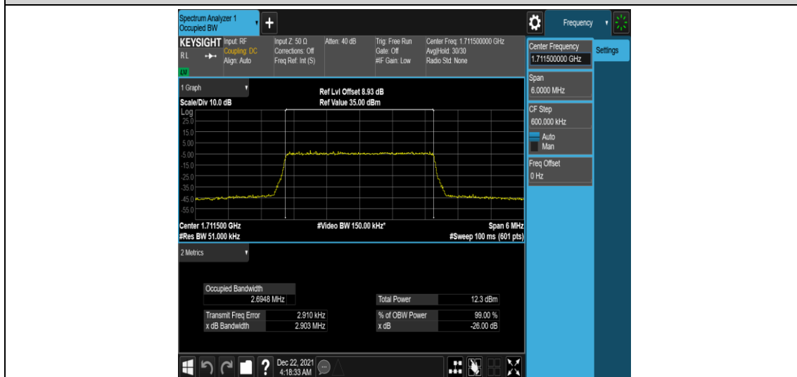
Band66-3MHz-16QAM-131987-15RB#0
