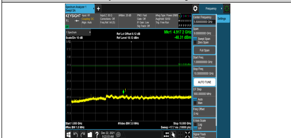
Band26-15MHz-QPSK-26865-1RB#0-Range4:1000~10000MHz
