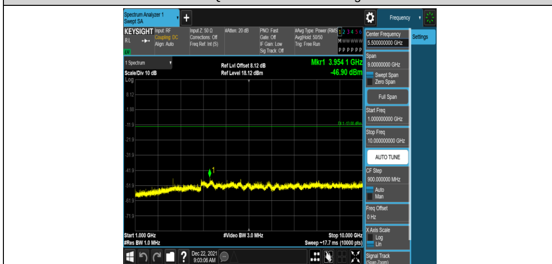
Band26-10MHz-16QAM-26915-1RB#0-Range4:1000~10000MHz
