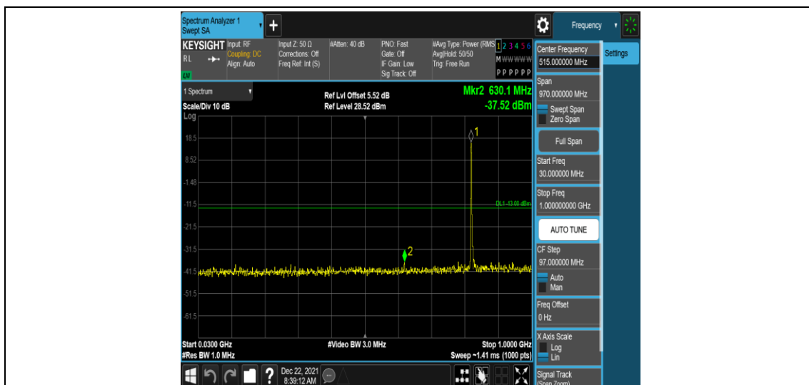
Band26-5MHz-QPSK-26815-1RB#0-Range3:30~1000MHz
