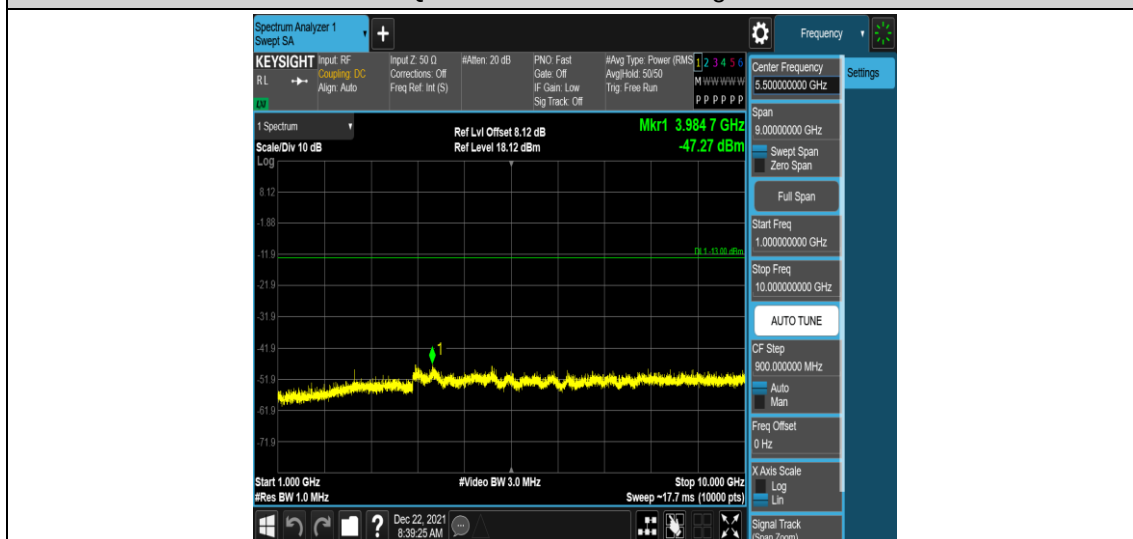
Band26-5MHz-QPSK-26815-1RB#0-Range4:1000~10000MHz
