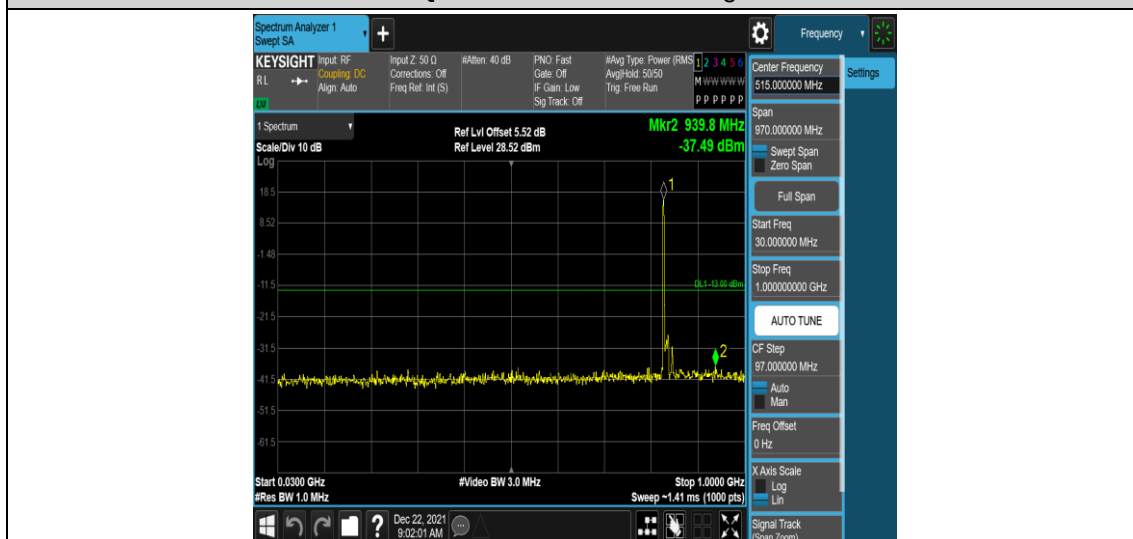
Band26-10MHz-QPSK-26915-1RB#0-Range3:30~1000MHz
