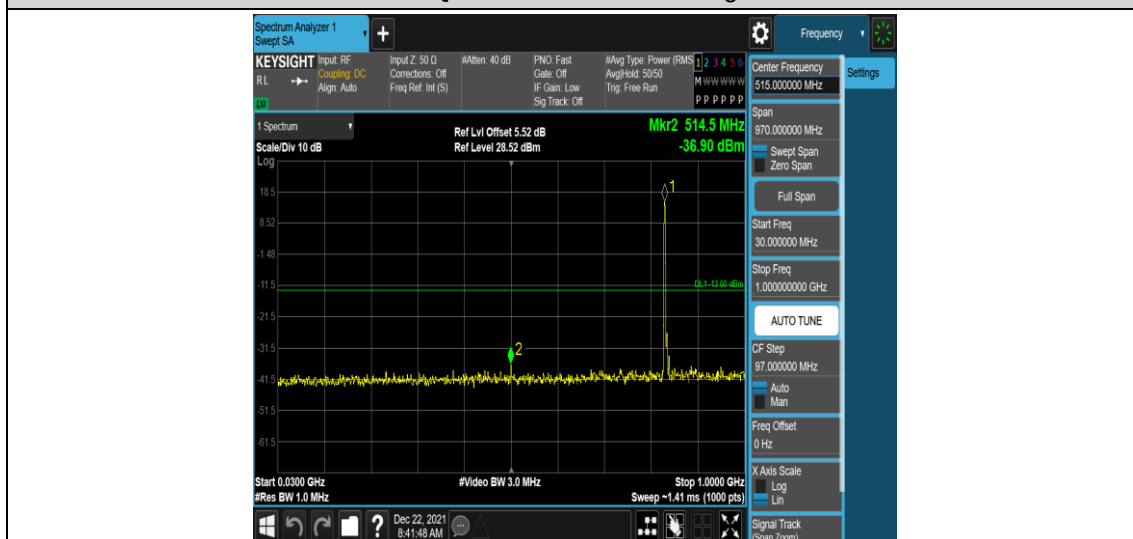
Band26-5MHz-16QAM-26915-1RB#0-Range3:30~1000MHz
