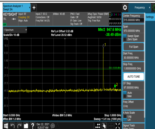
Band26-3MHz-QPSK-27025-1RB#0-Range3:30~1000MHz
