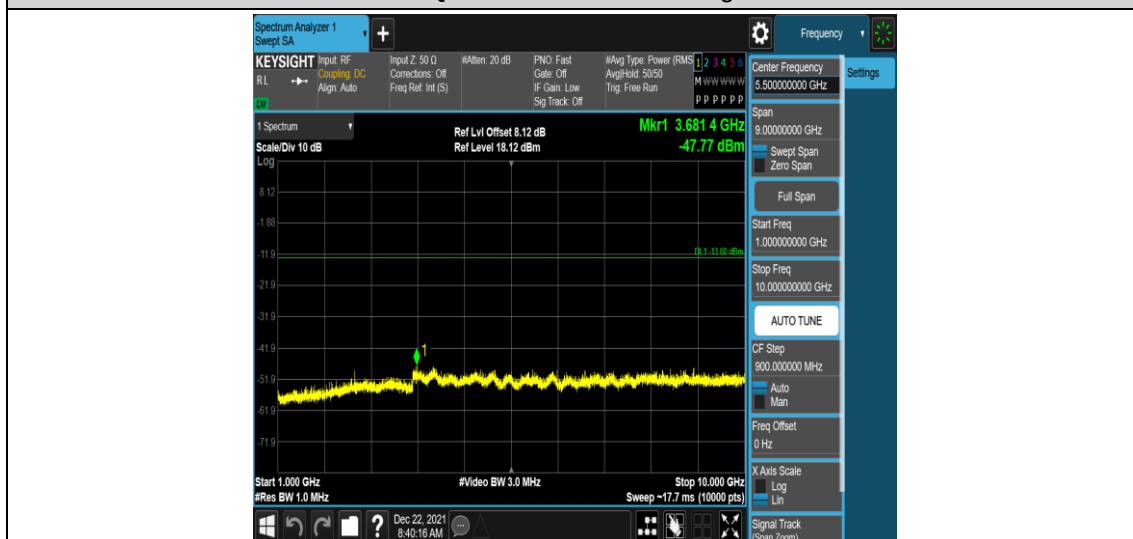
Band26-5MHz-16QAM-26815-1RB#0-Range4:1000~10000MHz
