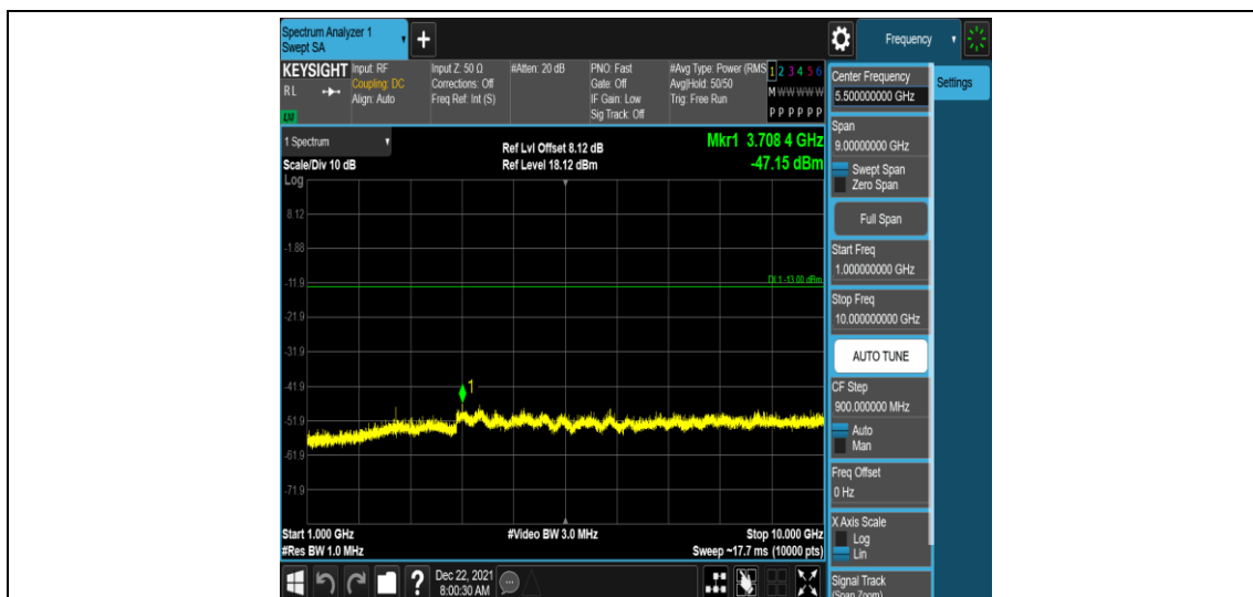
Band26-1.4MHz-QPSK-27033-1RB#0-Range4:1000~10000MHz
