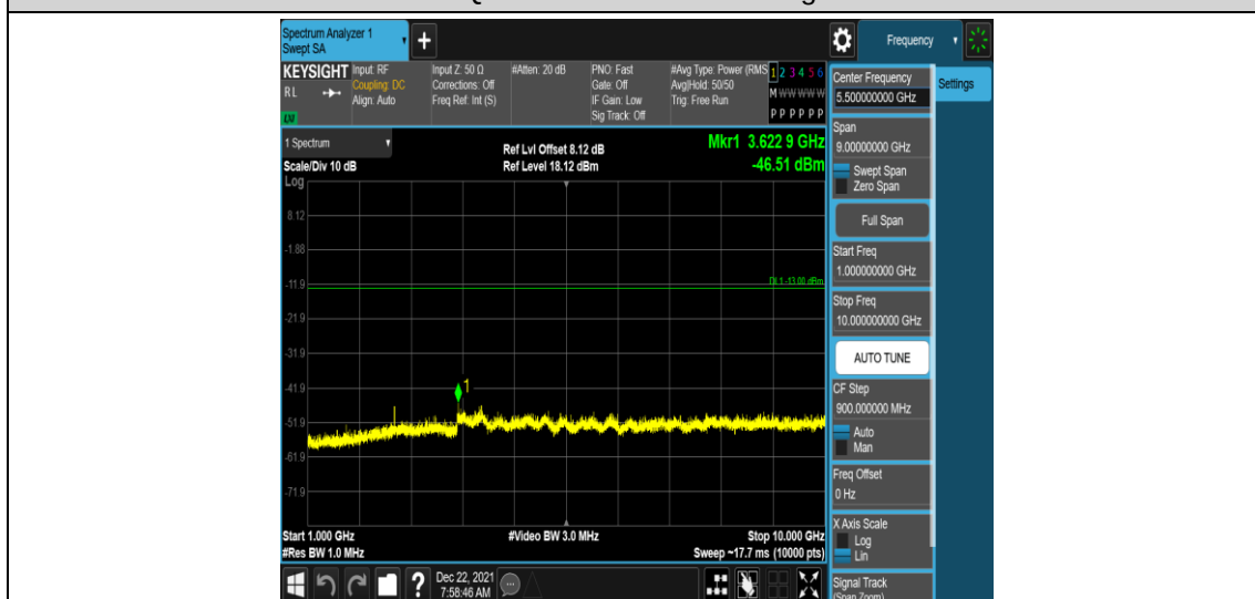
Band26-1.4MHz-QPSK-26915-1RB#0-Range4:1000~10000MHz
