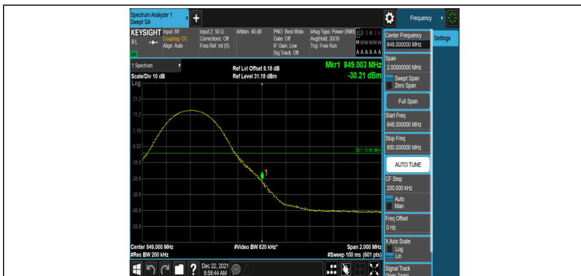
Band26-10MHz-QPSK-26990-1RB#49
