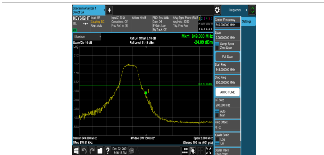
Band26-3MHz-16QAM-27025-1RB#14
