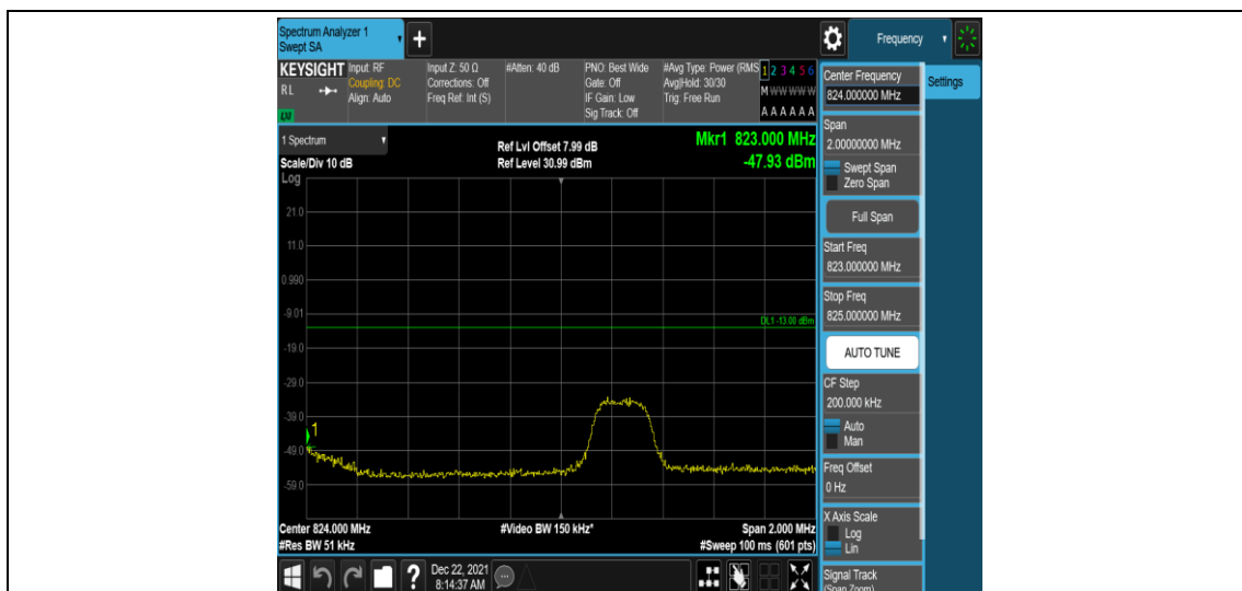
Band26-3MHz-16QAM-26805-1RB#14
