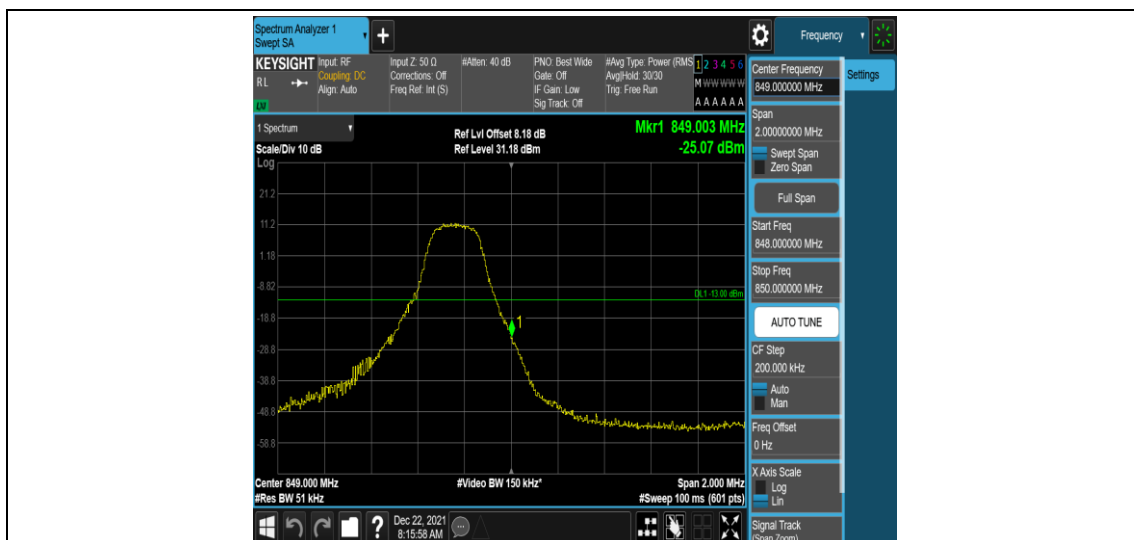
Band26-3MHz-QPSK-27025-1RB#14
