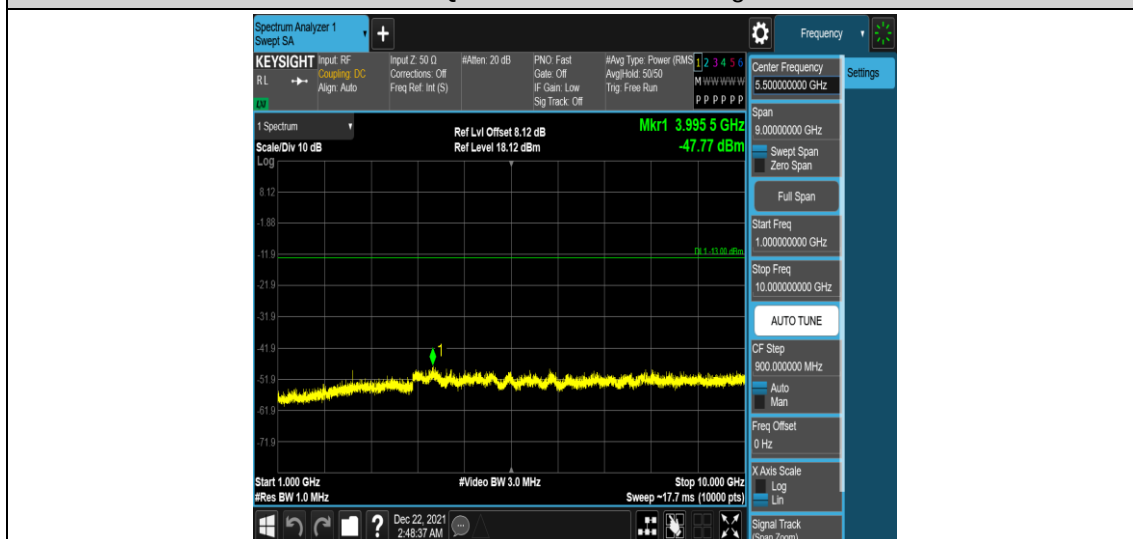
Band26-1.4MHz-16QAM-26697-1RB#0-Range4:1000~10000MHz
