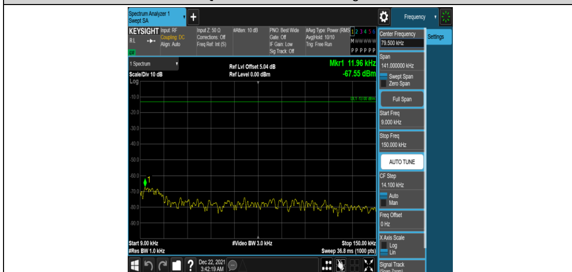
Band26-10MHz-QPSK-26740-1RB#0-Range1:0.009~0.15MHz
