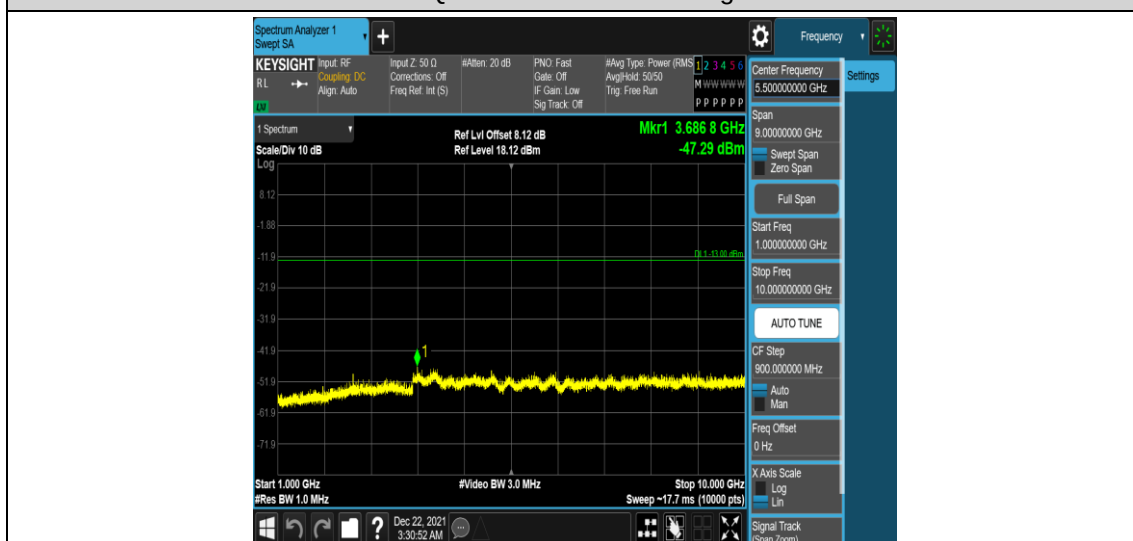
Band26-5MHz-16QAM-26740-1RB#0-Range4:1000~10000MHz
