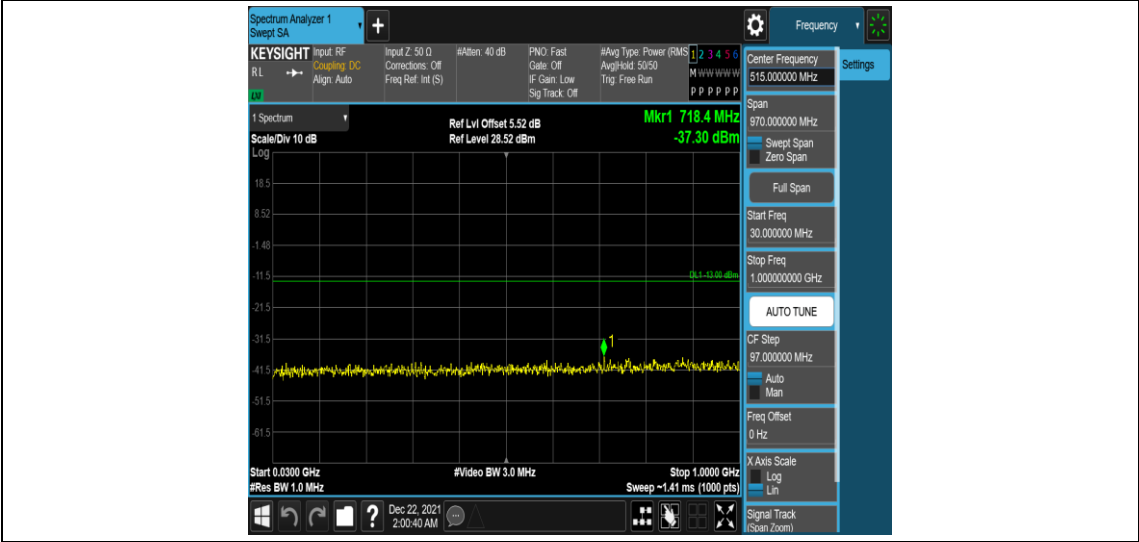
Band25-15MHz-QPSK-26115-1RB#0-Range3:30~1000MHz
