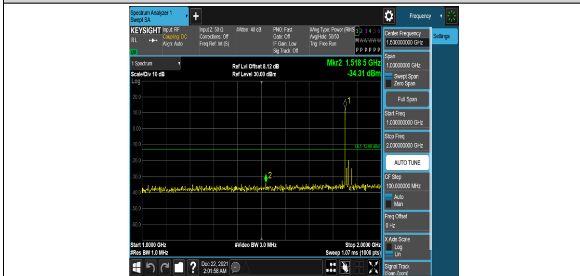
Band25-15MHz-16QAM-26115-1RB#0-Range4:1000~2000MHz
