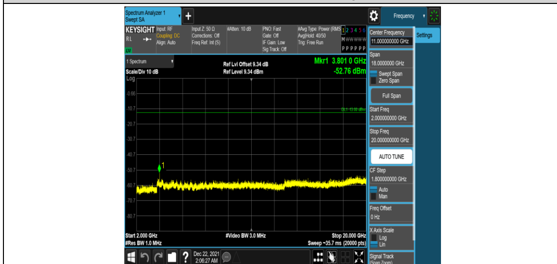
Band25-15MHz-16QAM-26615-1RB#0-Range5:2000~20000MHz
