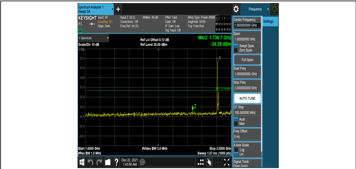
Band25-10MHz-16QAM-26640-1RB#0-Range4:1000~2000MHz
