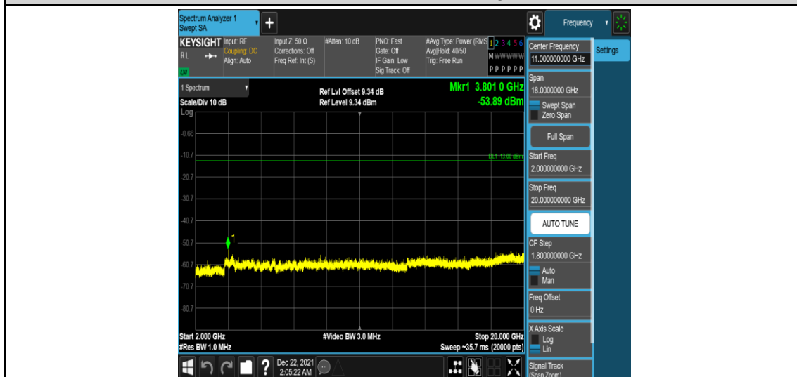
Band25-15MHz-QPSK-26615-1RB#0-Range5:2000~20000MHz
