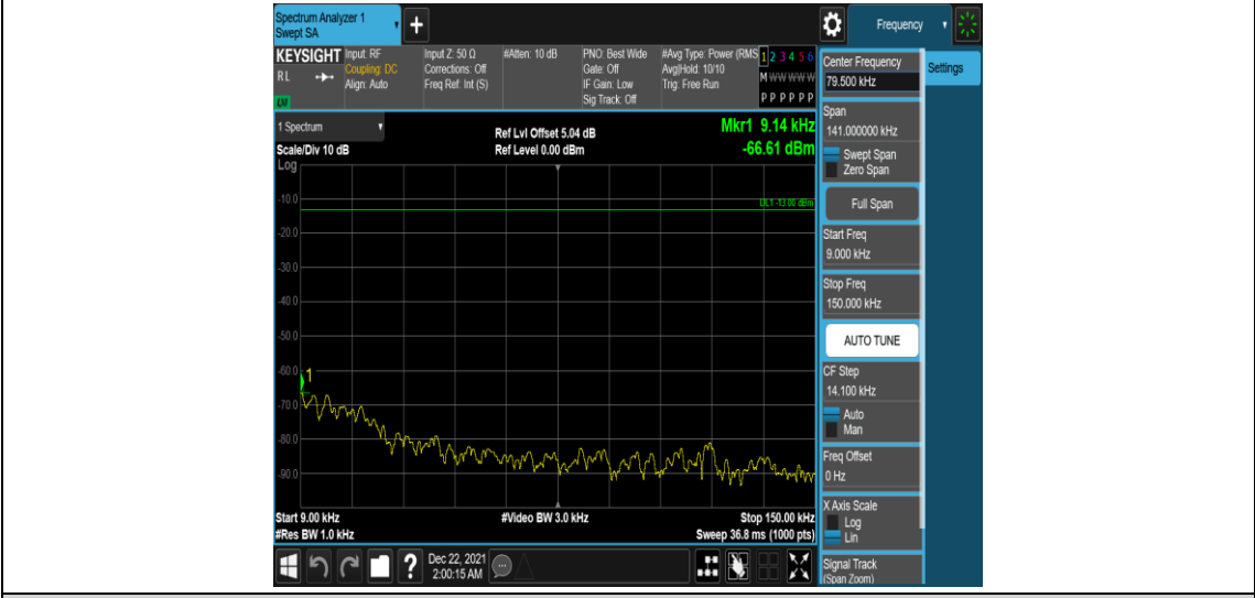
Band25-15MHz-QPSK-26115-1RB#0-Range1:0.009~0.15MHz
