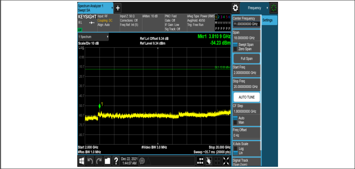
Band25-10MHz-16QAM-26640-1RB#0-Range5:2000~20000MHz
