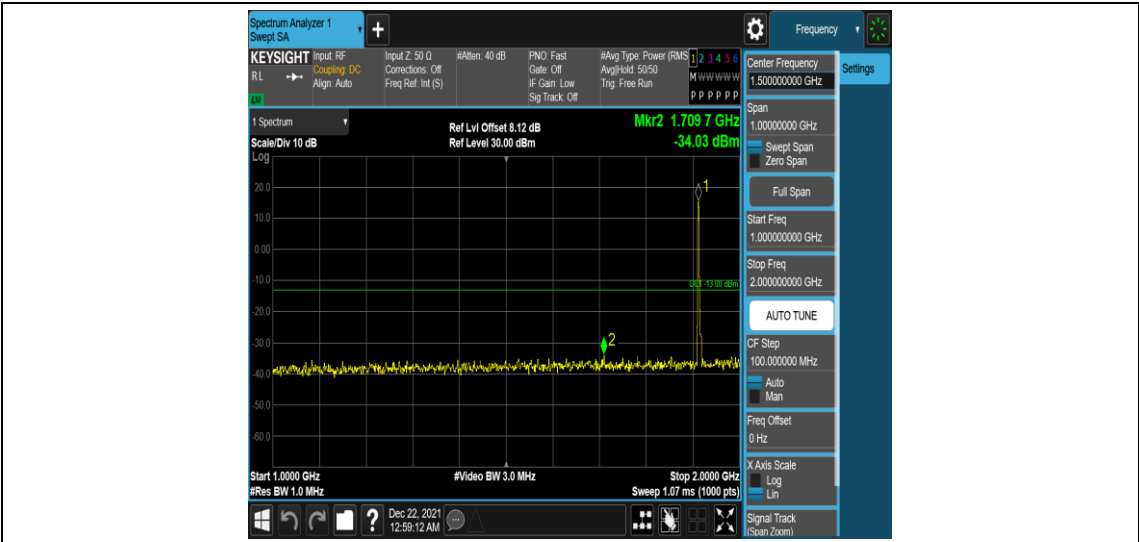
Band25-3MHz-16QAM-26675-1RB#0-Range4:1000~2000MHz
