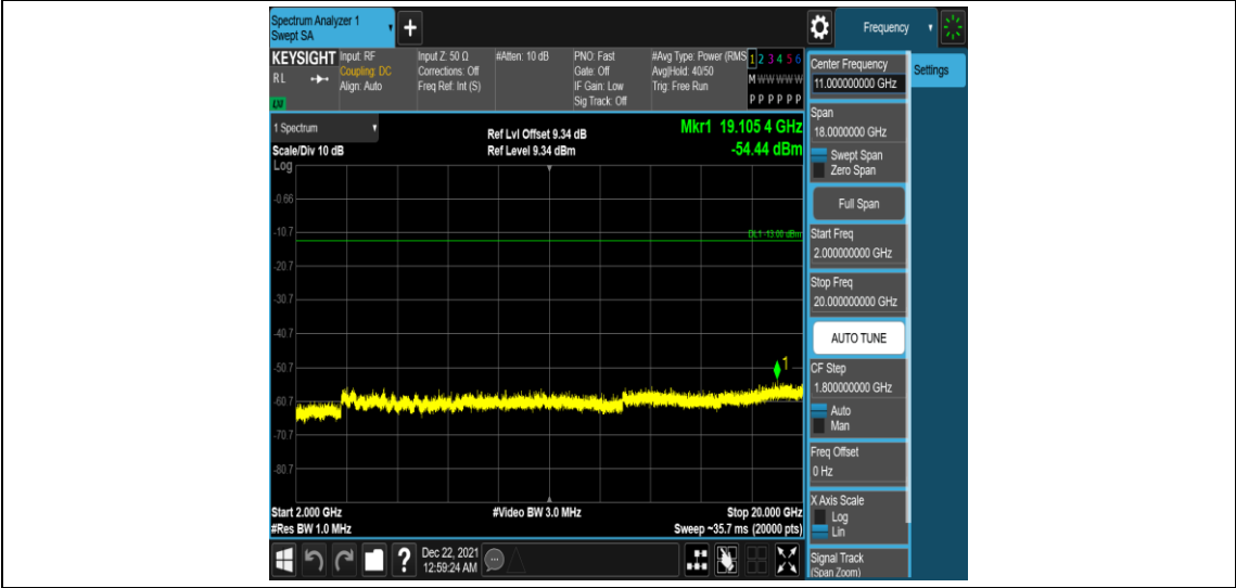
Band25-3MHz-16QAM-26675-1RB#0-Range5:2000~20000MHz
