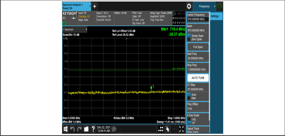
Band25-3MHz-16QAM-26055-1RB#0-Range3:30~1000MHz
