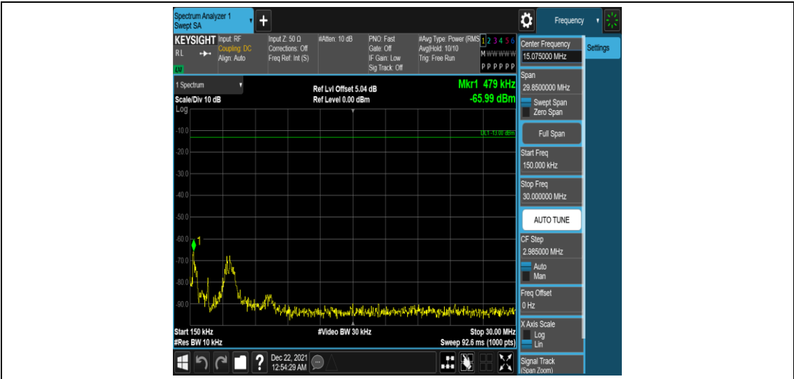
Band25-3MHz-16QAM-26055-1RB#0-Range2:0.15~30MHz
