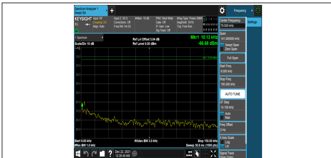
Band25-1.4MHz-QPSK-26683-1RB#0-Range1:0.009~0.15MHz
