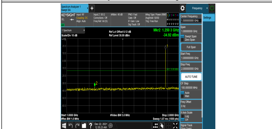
Band25-1.4MHz-16QAM-26365-1RB#0-Range4:1000~2000MHz
