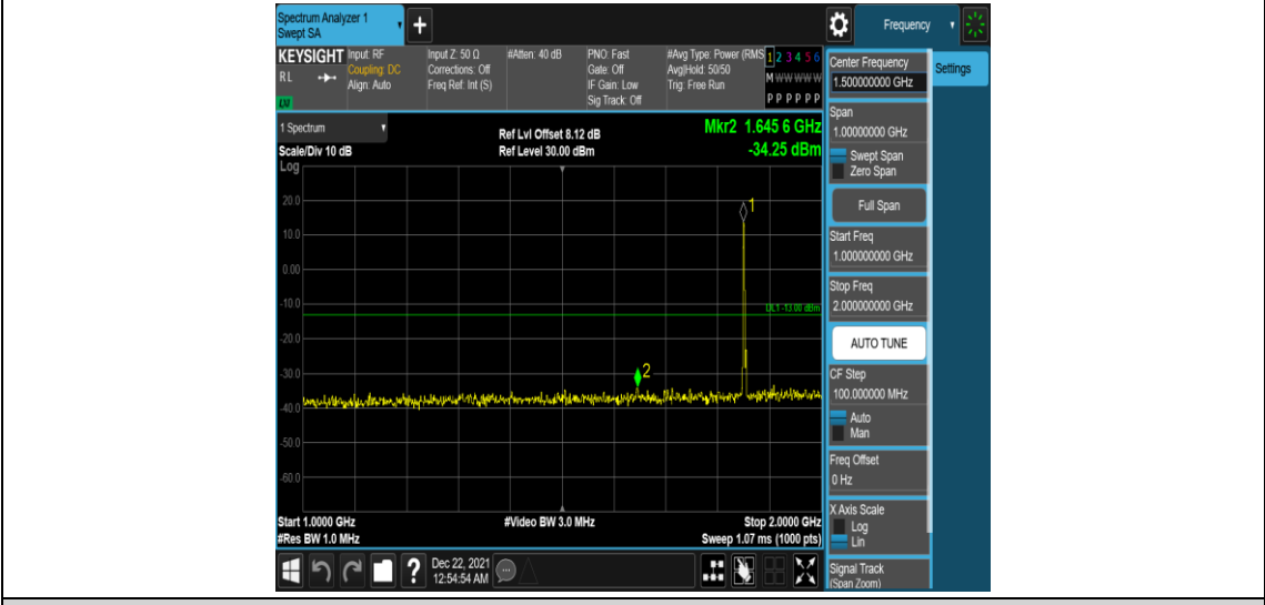
Band25-3MHz-16QAM-26055-1RB#0-Range4:1000~2000MHz
