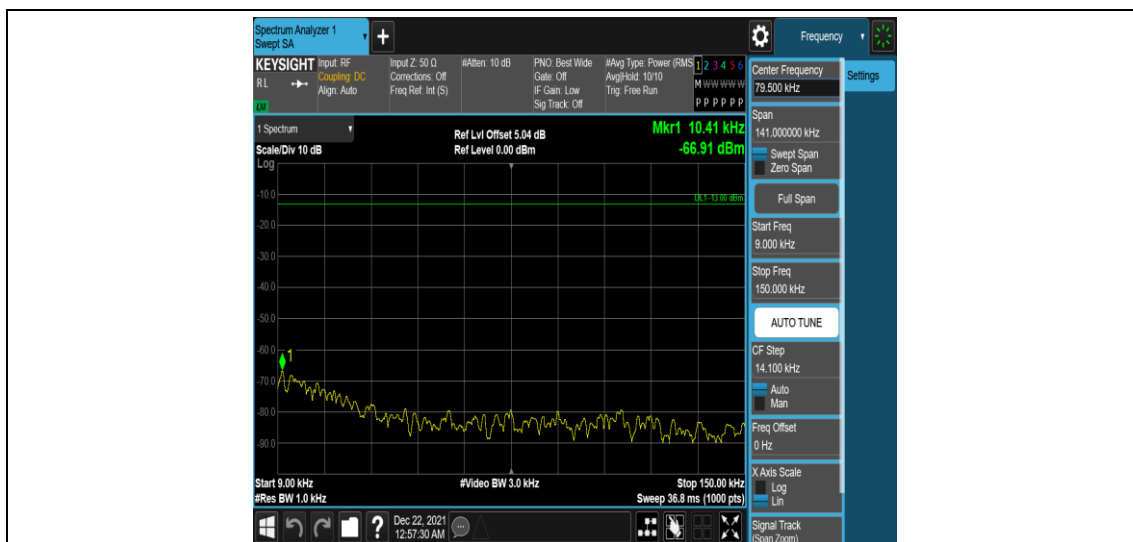
Band25-3MHz-QPSK-26675-1RB#0-Range1:0.009~0.15MHz
