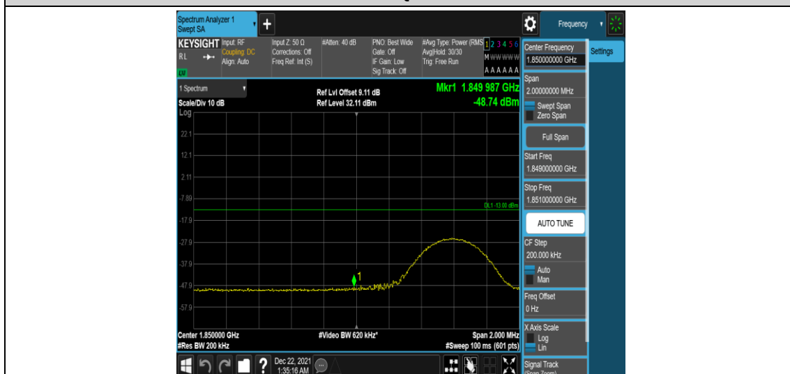
Band25-10MHz-16QAM-26090-1RB#49
