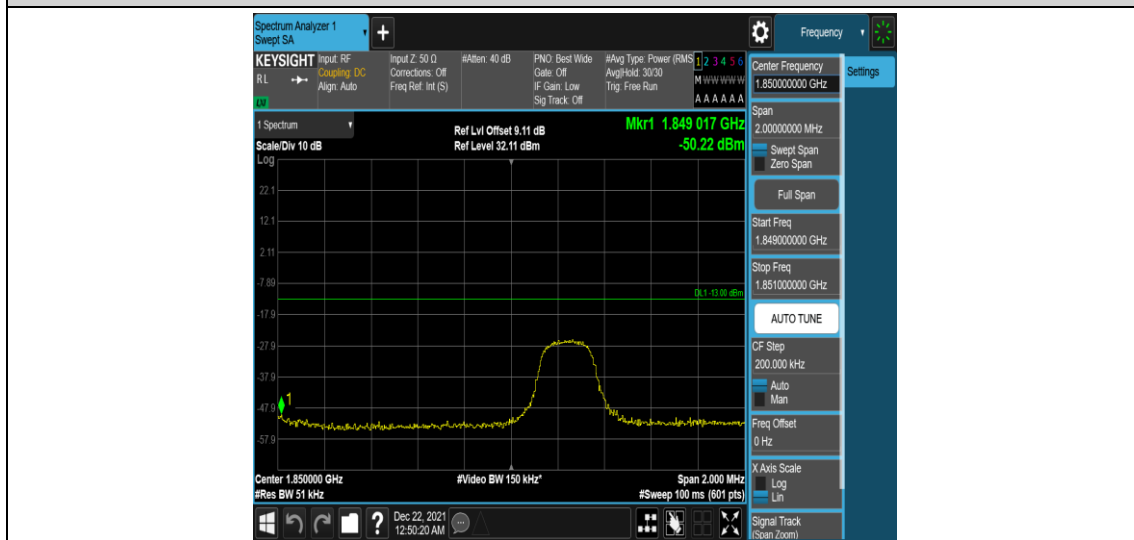
Band25-3MHz-QPSK-26055-1RB#14
