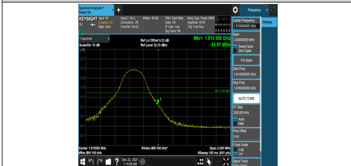
Band25-5MHz-16QAM-26665-1RB#24
