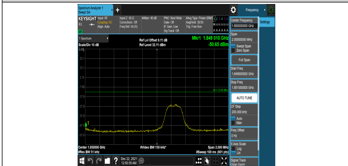
Band25-3MHz-16QAM-26055-1RB#14
