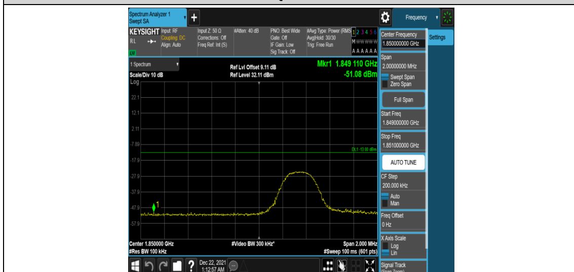
Band25-5MHz-QPSK-26065-1RB#24
