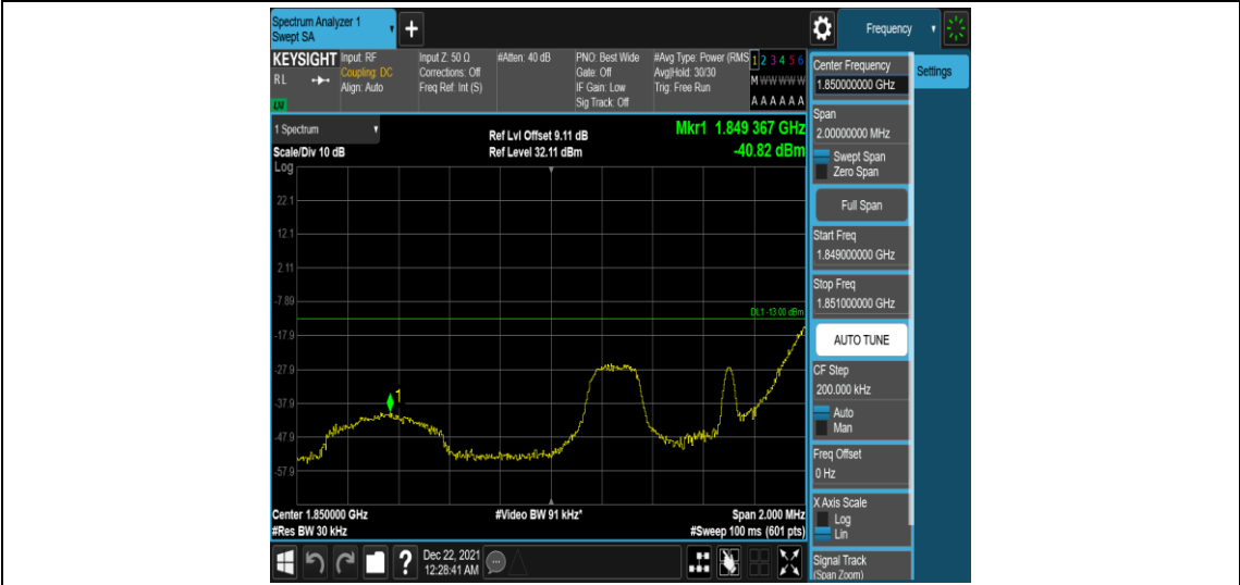
Band25-1.4MHz-QPSK-26047-1RB#5
