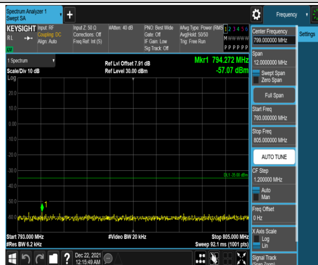
Band13-10MHz-16QAM-23230-1RB#0-Range6:793~805MHz
