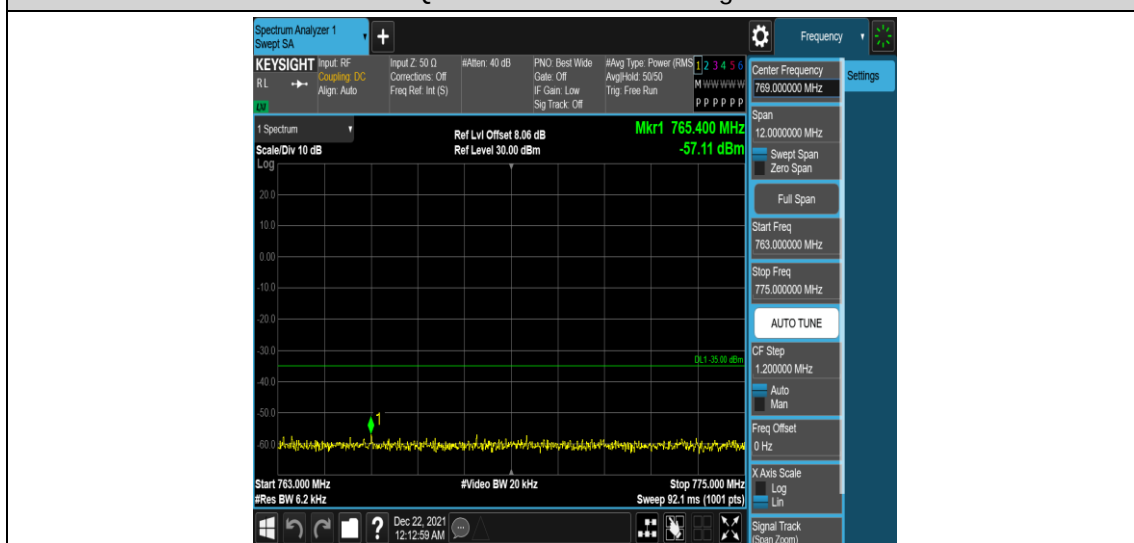
Band13-10MHz-QPSK-23230-1RB#0-Range5:763~775MHz
