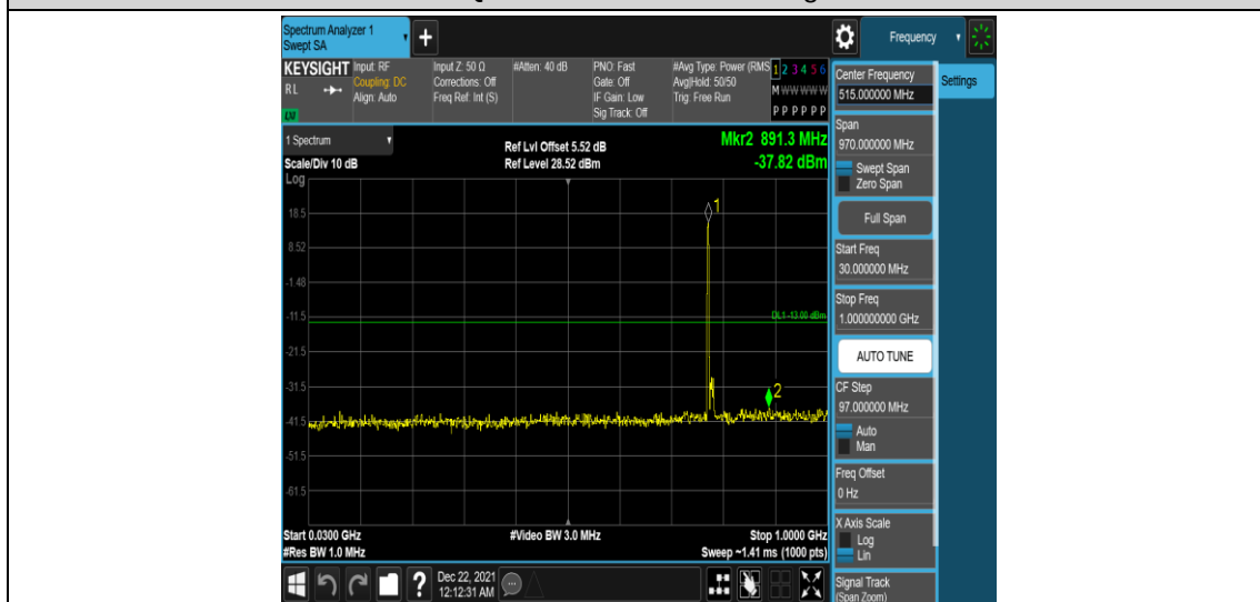
Band13-10MHz-QPSK-23230-1RB#0-Range3:30~1000MHz
