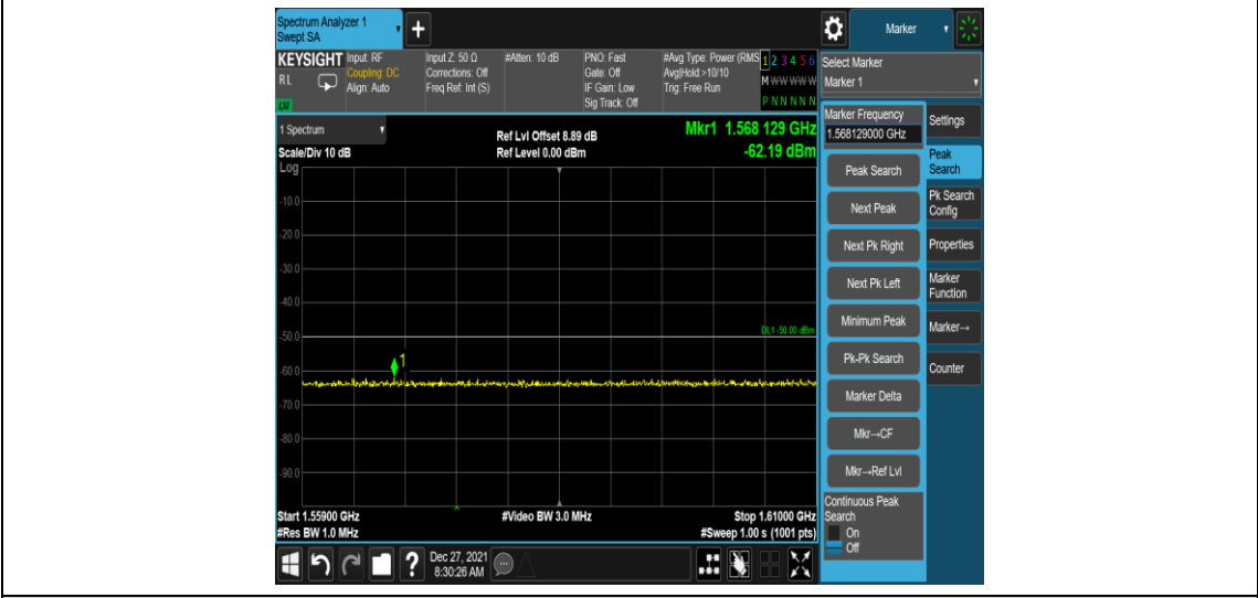
Band13-5MHz-16QAM-23255-1RB#0-Range7:1559~1610MHz
