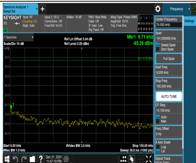
Band13-5MHz-16QAM-23255-1RB#0-Range1:0.009~0.15MHz
