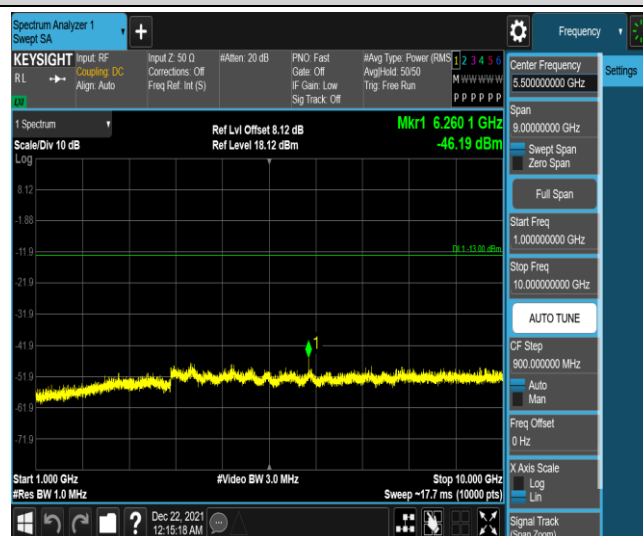
Band13-10MHz-16QAM-23230-1RB#0-Range4:1000~10000MHz
