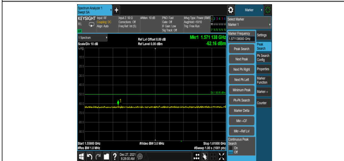
Band13-5MHz-QPSK-23255-1RB#0-Range7:1559~1610MHz
