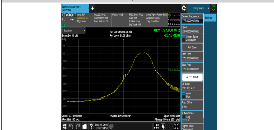
Band13-5MHz-16QAM-23205-1RB#0
