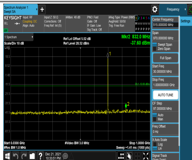
Band12-3MHz-16QAM-23095-1RB#0-Range3:30~1000MHz
