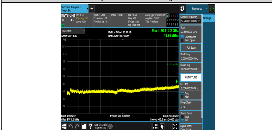
Band7-20MHz-16QAM-20850-1RB#0-Range5:3000~26500MHz
