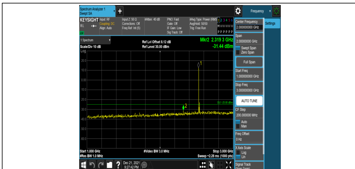
Band7-15MHz-QPSK-21100-1RB#0-Range4:1000~3000MHz
