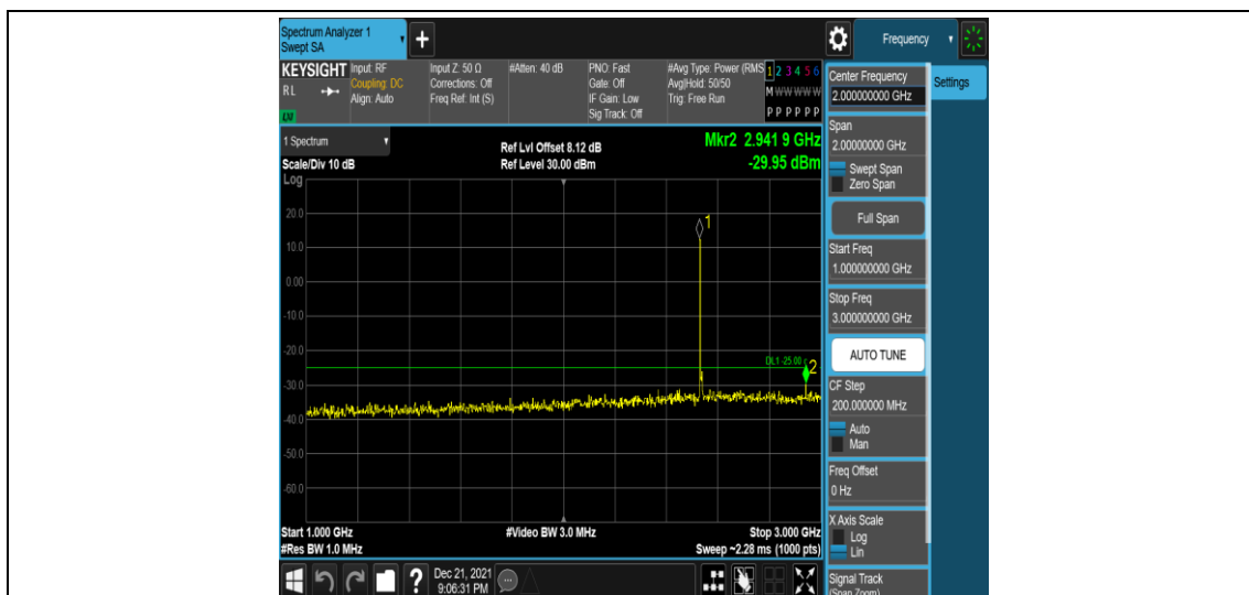
Band7-10MHz-16QAM-21100-1RB#0-Range4:1000~3000MHz
