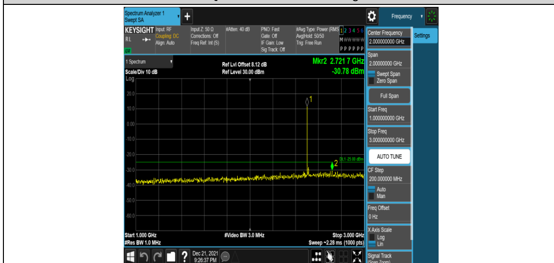
Band7-15MHz-16QAM-20825-1RB#0-Range4:1000~3000MHz
