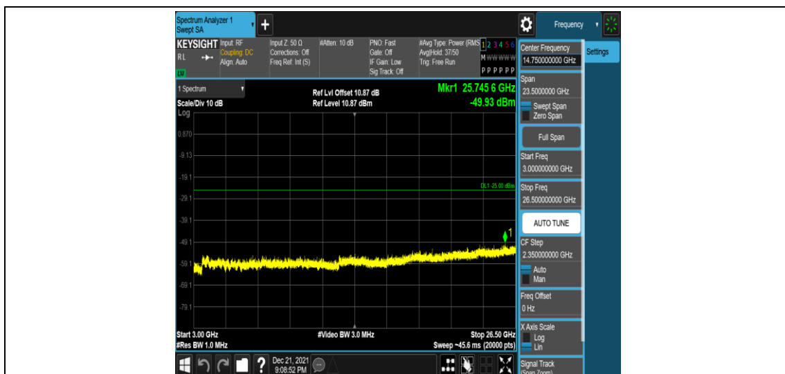
Band7-10MHz-16QAM-21400-1RB#0-Range5:3000~26500MHz
