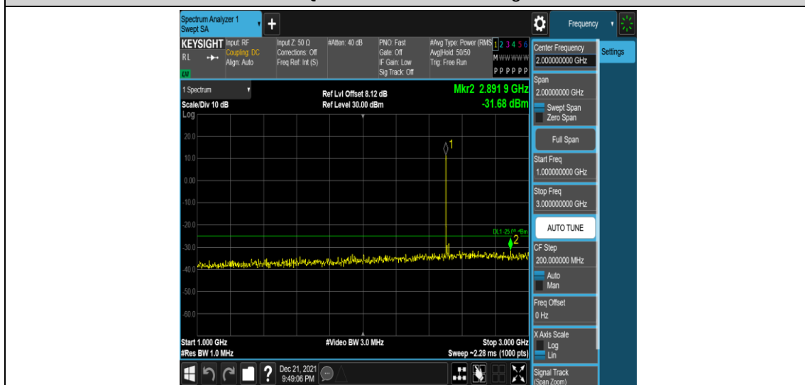
Band7-20MHz-16QAM-20850-1RB#0-Range4:1000~3000MHz
