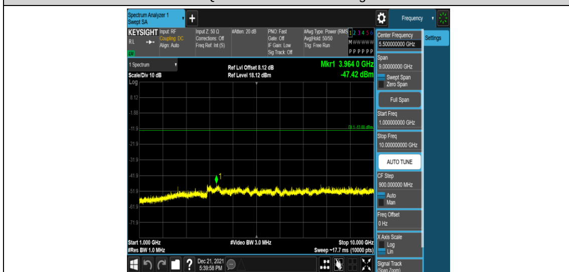
Band5-1.4MHz-QPSK-20407-1RB#0-Range4:1000~10000MHz
