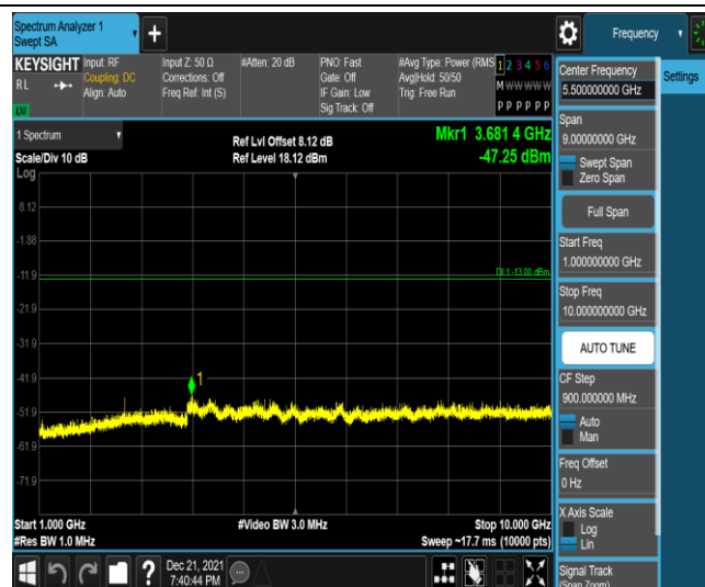
Band5-3MHz-QPSK-20525-1RB#0-Range4:1000~10000MHz
