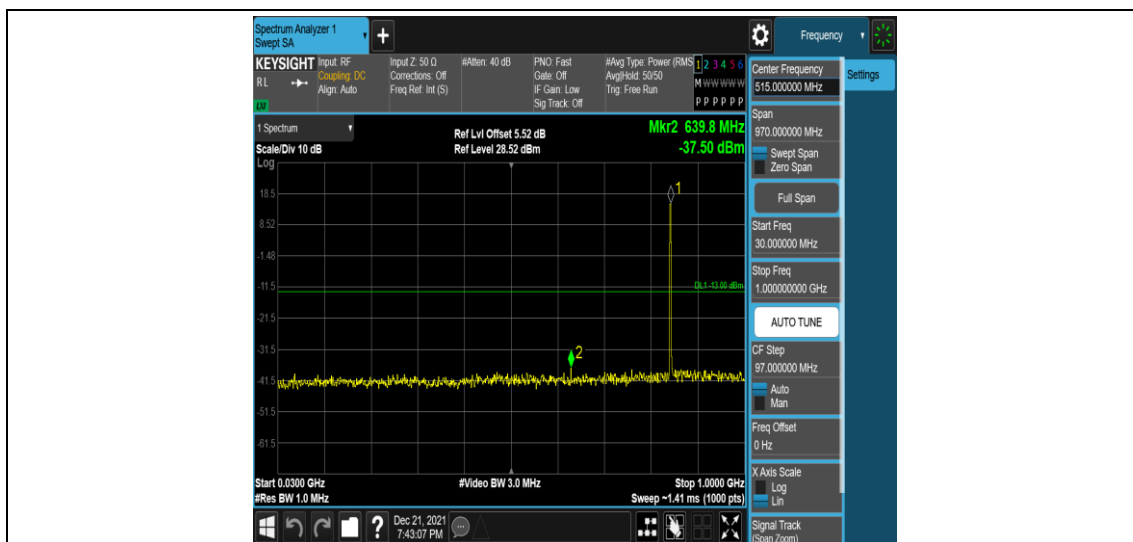
Band5-3MHz-16QAM-20635-1RB#0-Range3:30~1000MHz
