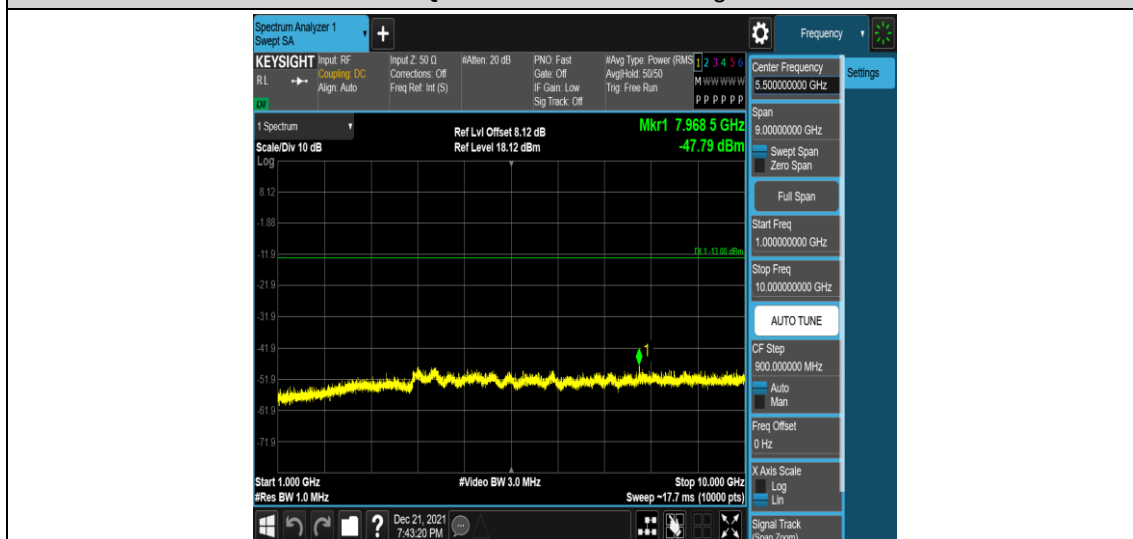
Band5-3MHz-16QAM-20635-1RB#0-Range4:1000~10000MHz
