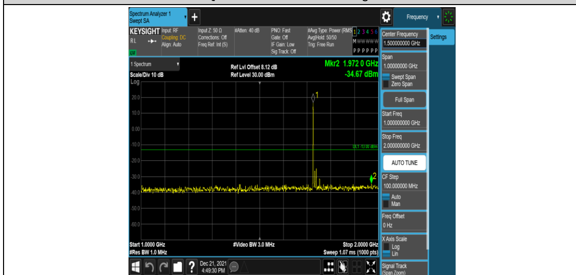
Band4-15MHz-QPSK-20175-1RB#0-Range4:1000~2000MHz
