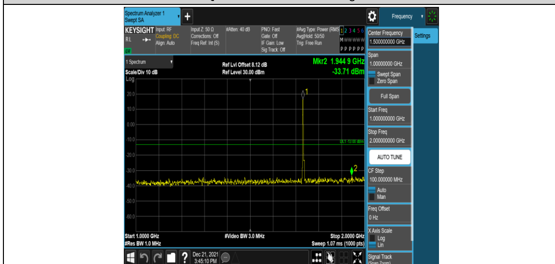
Band4-3MHz-16QAM-20175-1RB#0-Range4:1000~2000MHz
