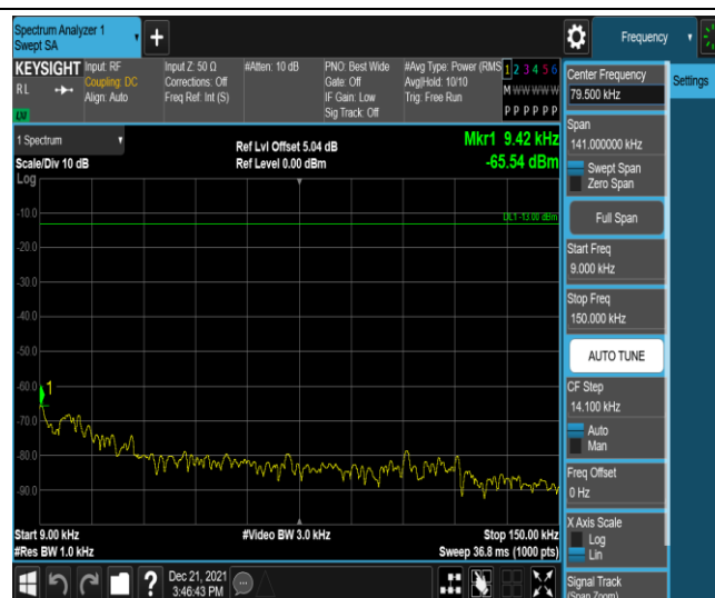
Band4-3MHz-16QAM-20385-1RB#0-Range1:0.009~0.15MHz
