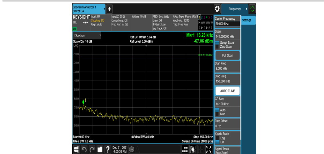
Band4-5MHz-QPSK-20175-1RB#0-Range1:0.009~0.15MHz
