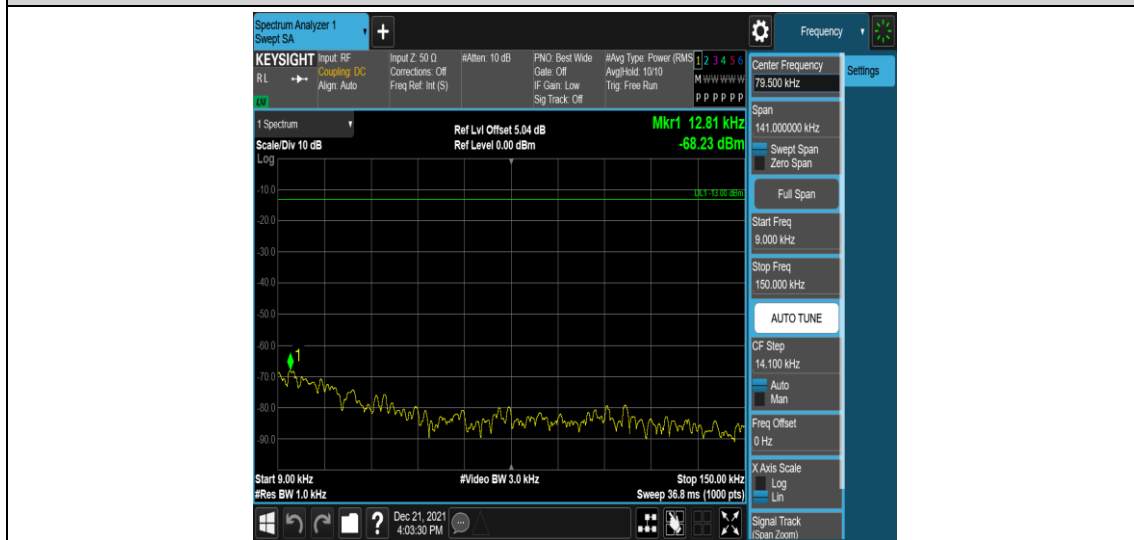
Band4-5MHz-QPSK-19975-1RB#0-Range1:0.009~0.15MHz
