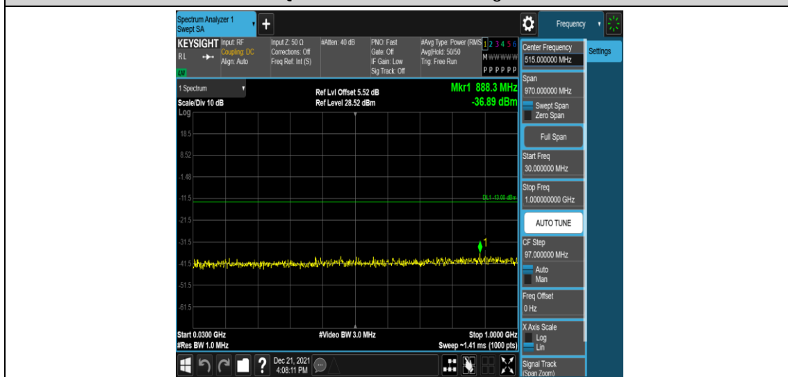
Band4-5MHz-QPSK-20375-1RB#0-Range3:30~1000MHz
