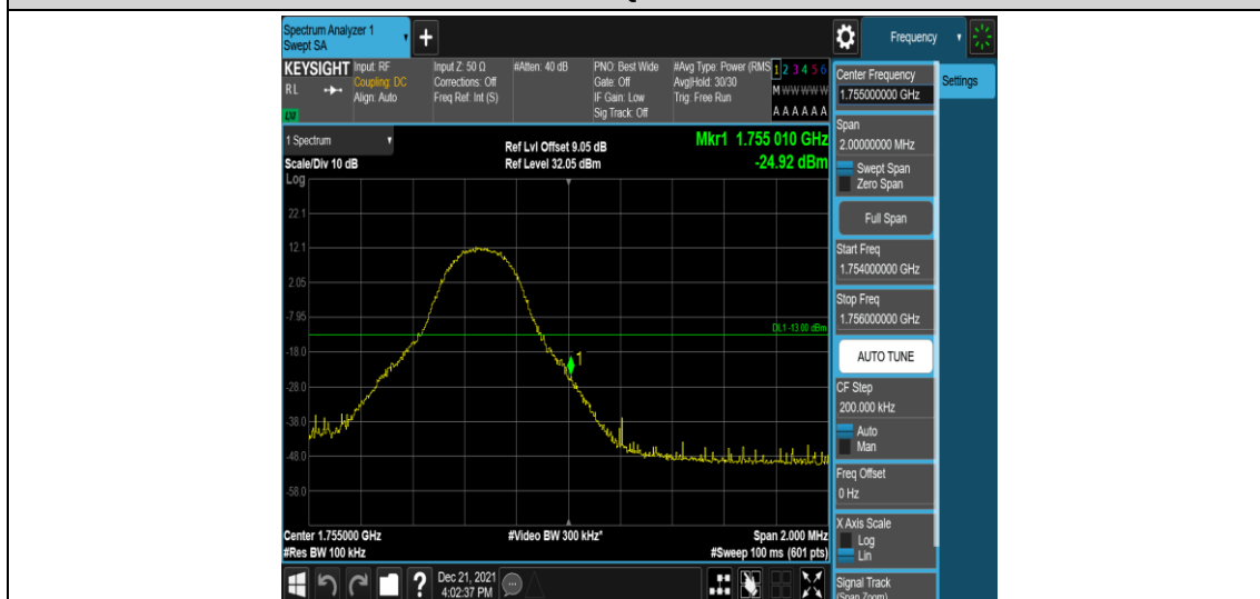
Band4-5MHz-16QAM-20375-1RB#24
