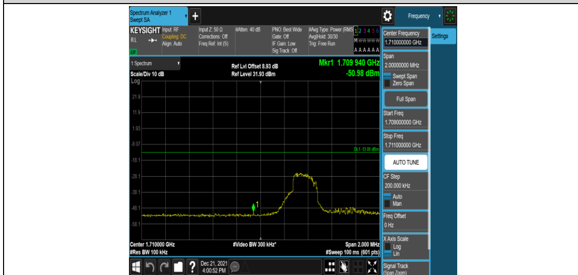
Band4-5MHz-16QAM-19975-1RB#24
