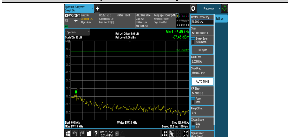
Band2-20MHz-QPSK-18900-1RB#0-Range1:0.009~0.15MHz
