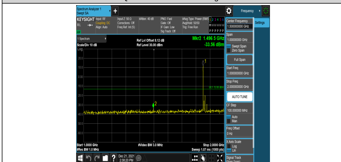
Band2-15MHz-QPSK-18675-1RB#0-Range4:1000~2000MHz
