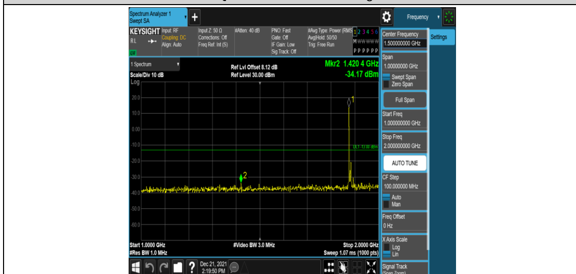
Band2-10MHz-16QAM-18900-1RB#0-Range4:1000~2000MHz
