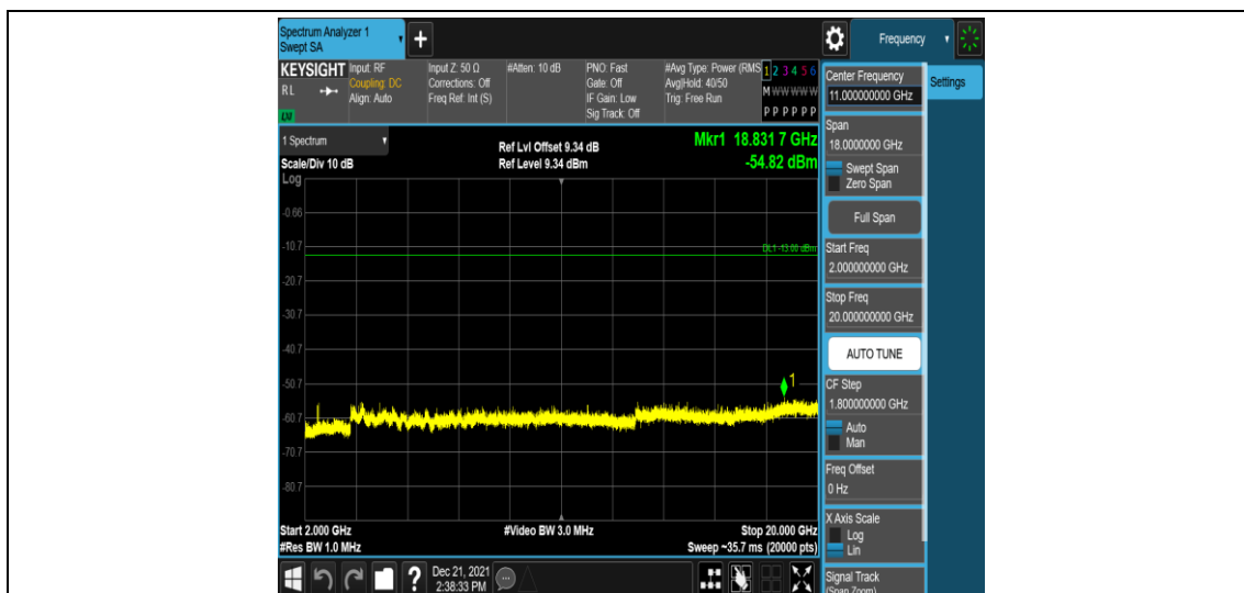
Band2-15MHz-QPSK-18675-1RB#0-Range5:2000~20000MHz
