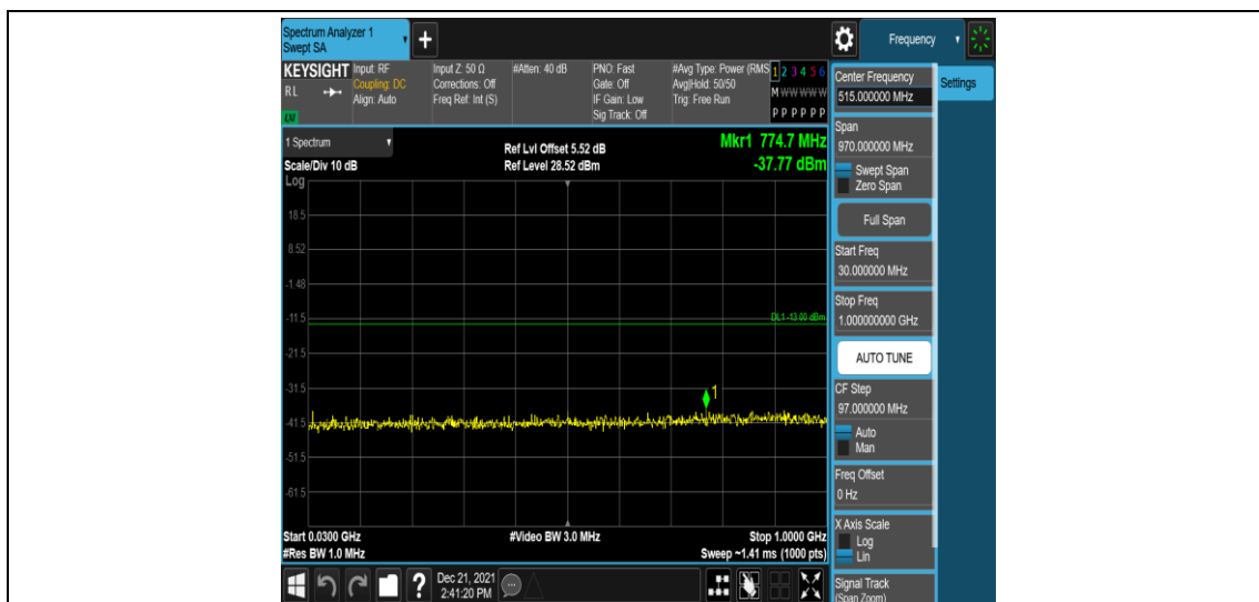
Band2-15MHz-16QAM-18900-1RB#0-Range3:30~1000MHz
