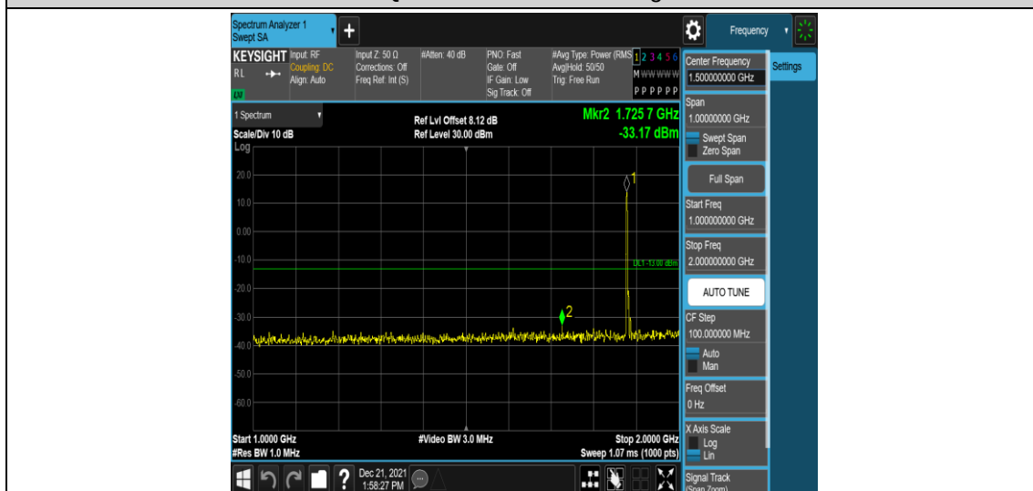
Band2-5MHz-16QAM-18900-1RB#0-Range4:1000~2000MHz
