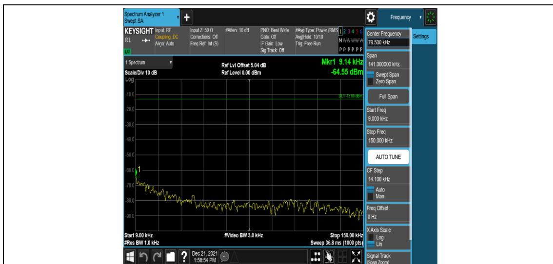
Band2-5MHz-QPSK-19175-1RB#0-Range1:0.009~0.15MHz
