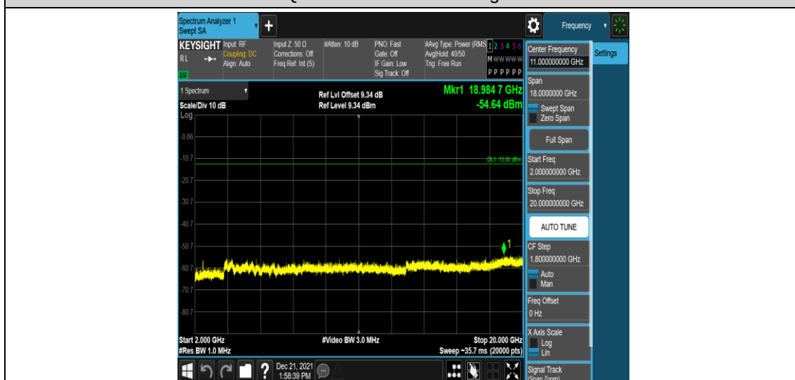
Band2-5MHz-16QAM-18900-1RB#0-Range5:2000~20000MHz
