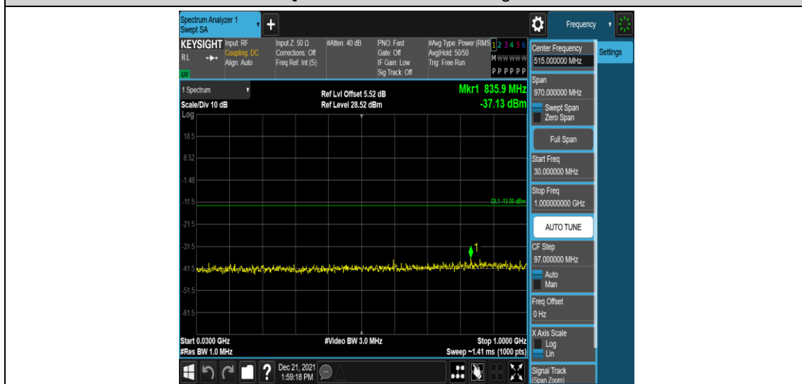
Band2-5MHz-QPSK-19175-1RB#0-Range3:30~1000MHz
