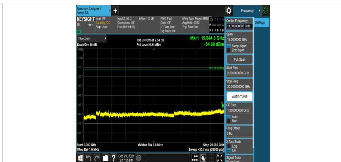
Band2-10MHz-16QAM-18650-1RB#0-Range5:2000~20000MHz
