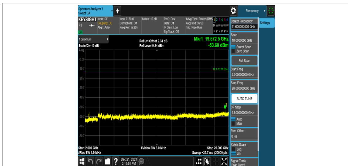
Band2-10MHz-QPSK-18650-1RB#0-Range5:2000~20000MHz
