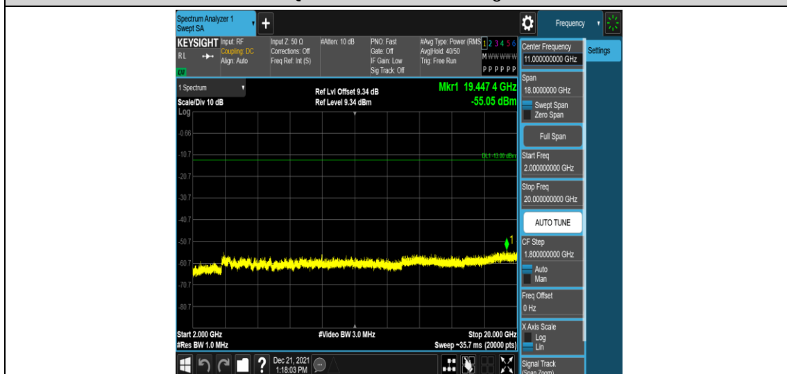
Band2-1.4MHz-16QAM-19193-1RB#0-Range5:2000~20000MHz
