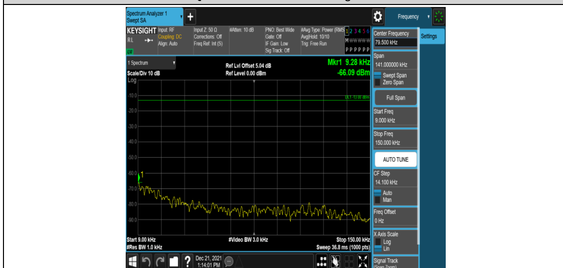
Band2-1.4MHz-QPSK-18900-1RB#0-Range1:0.009~0.15MHz
