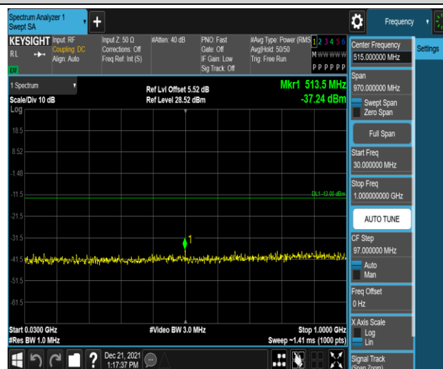
Band2-1.4MHz-16QAM-19193-1RB#0-Range3:30~1000MHz
