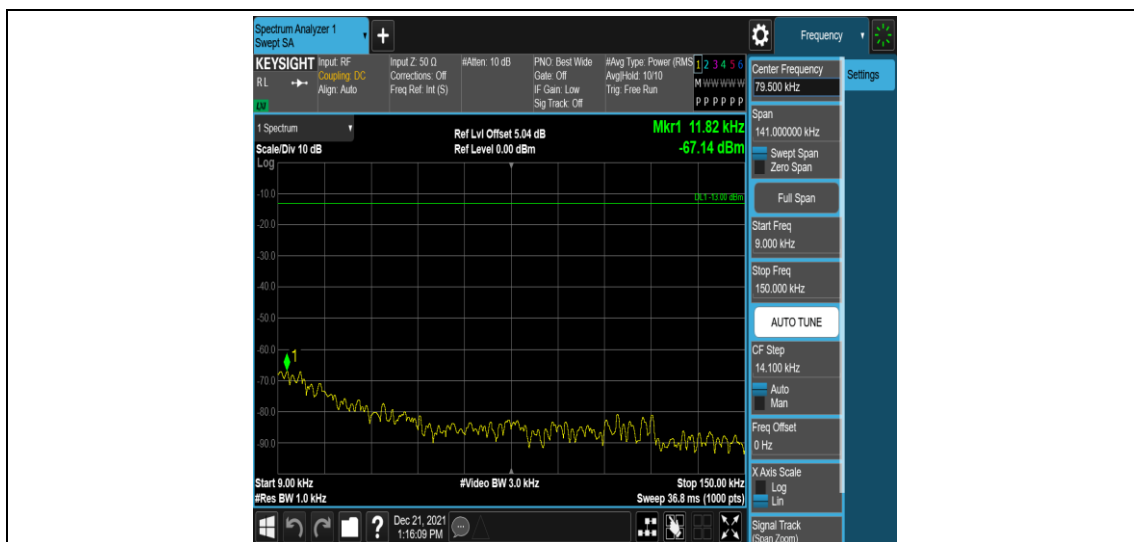
Band2-1.4MHz-QPSK-19193-1RB#0-Range1:0.009~0.15MHz
