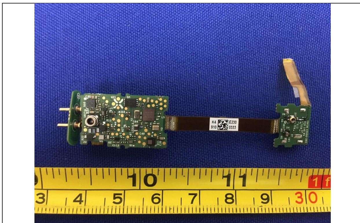
EUT Main board Rear View
