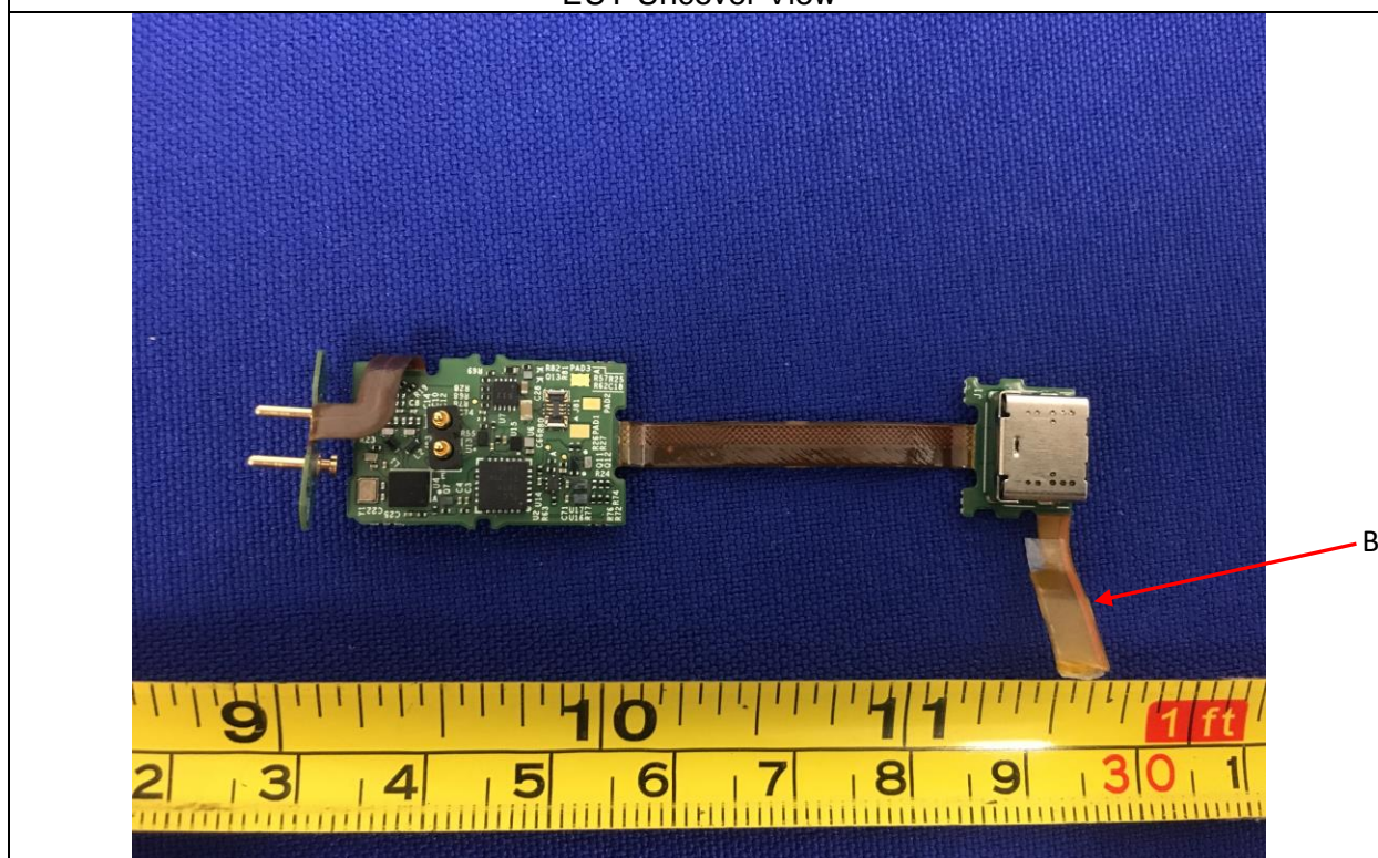
EUT Main board Front View
